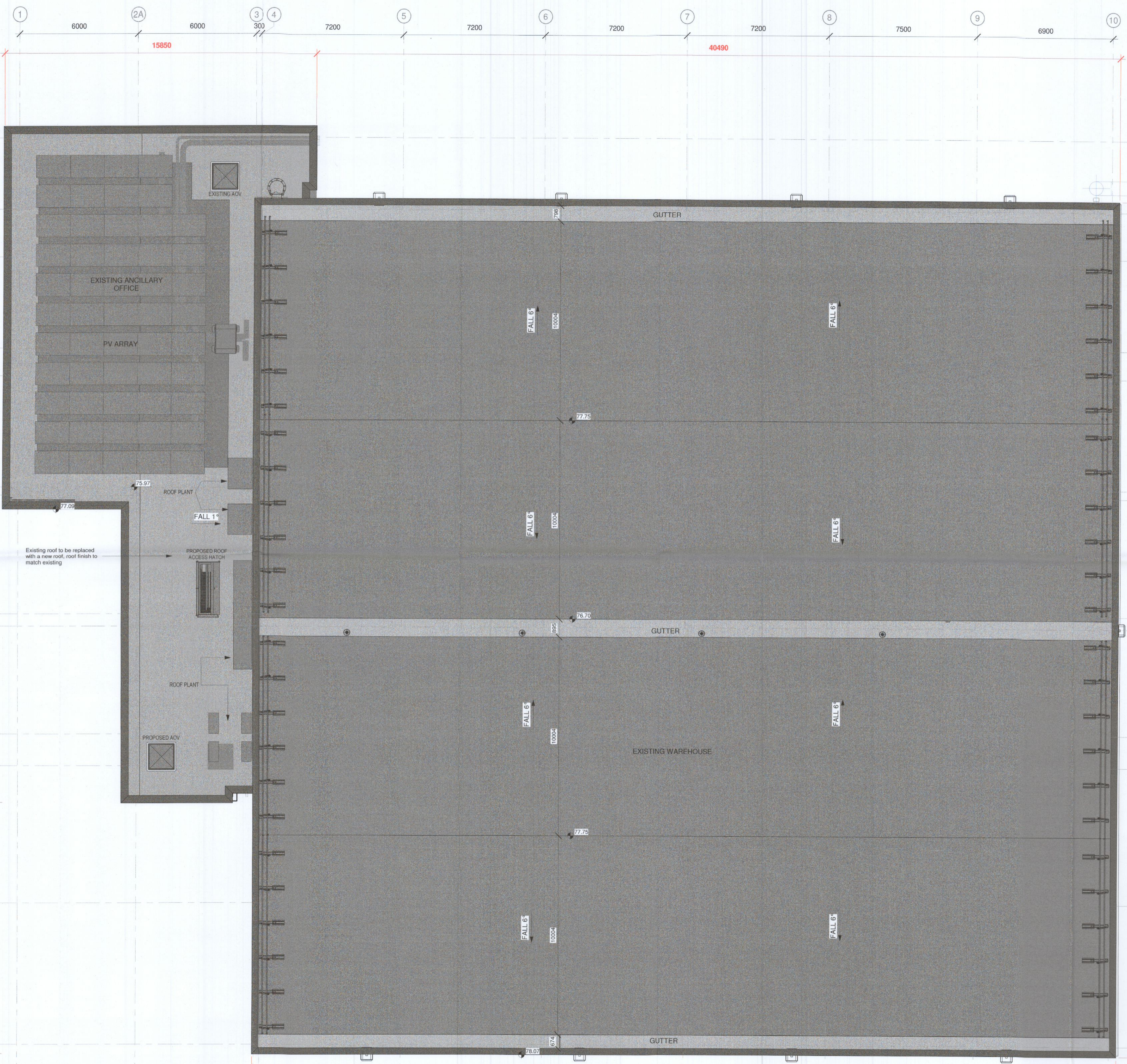
1 2016 Proposed Roof Level 1 : 100
