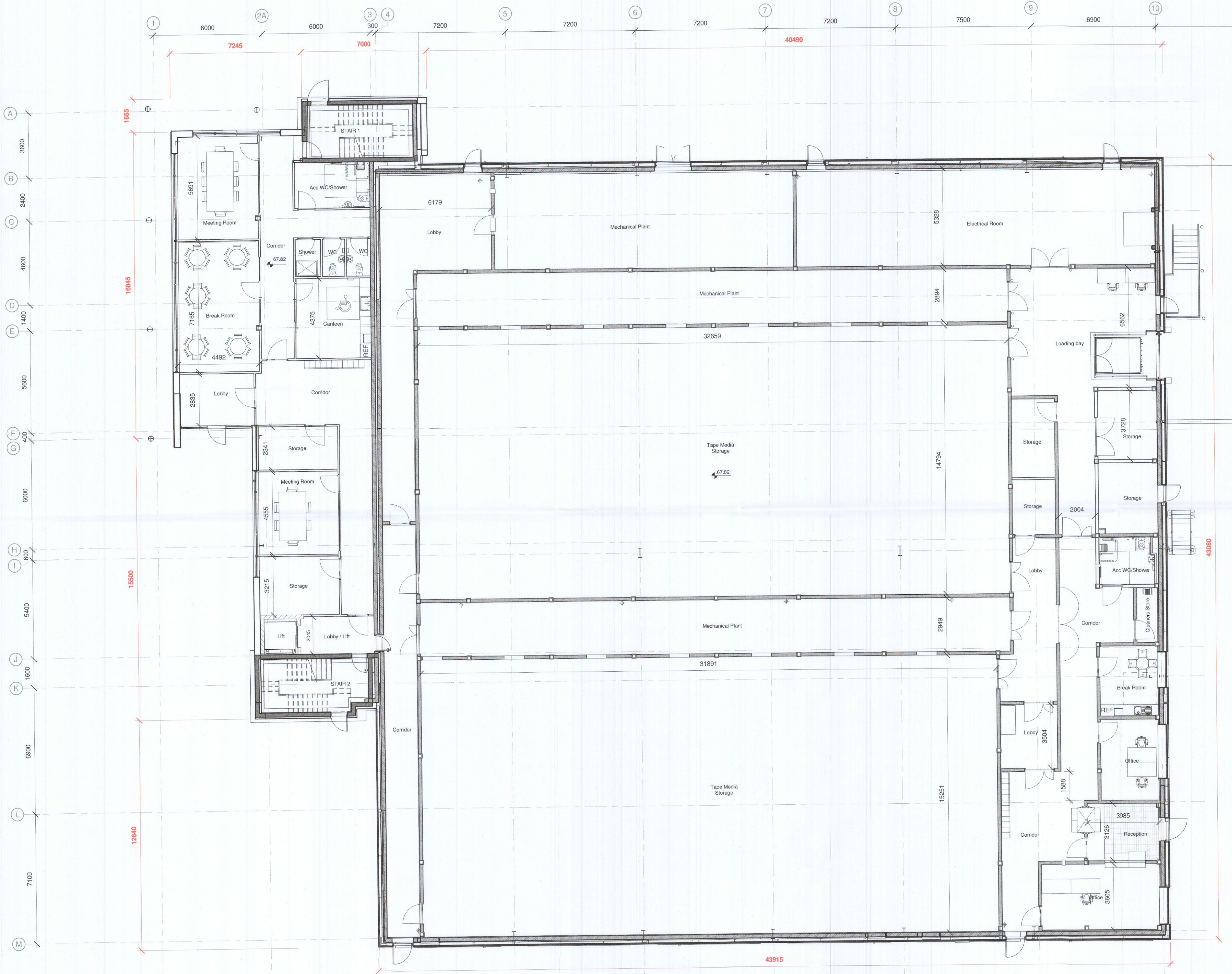
1 2004 Proposed Ground Floor Plan 1 : 100
