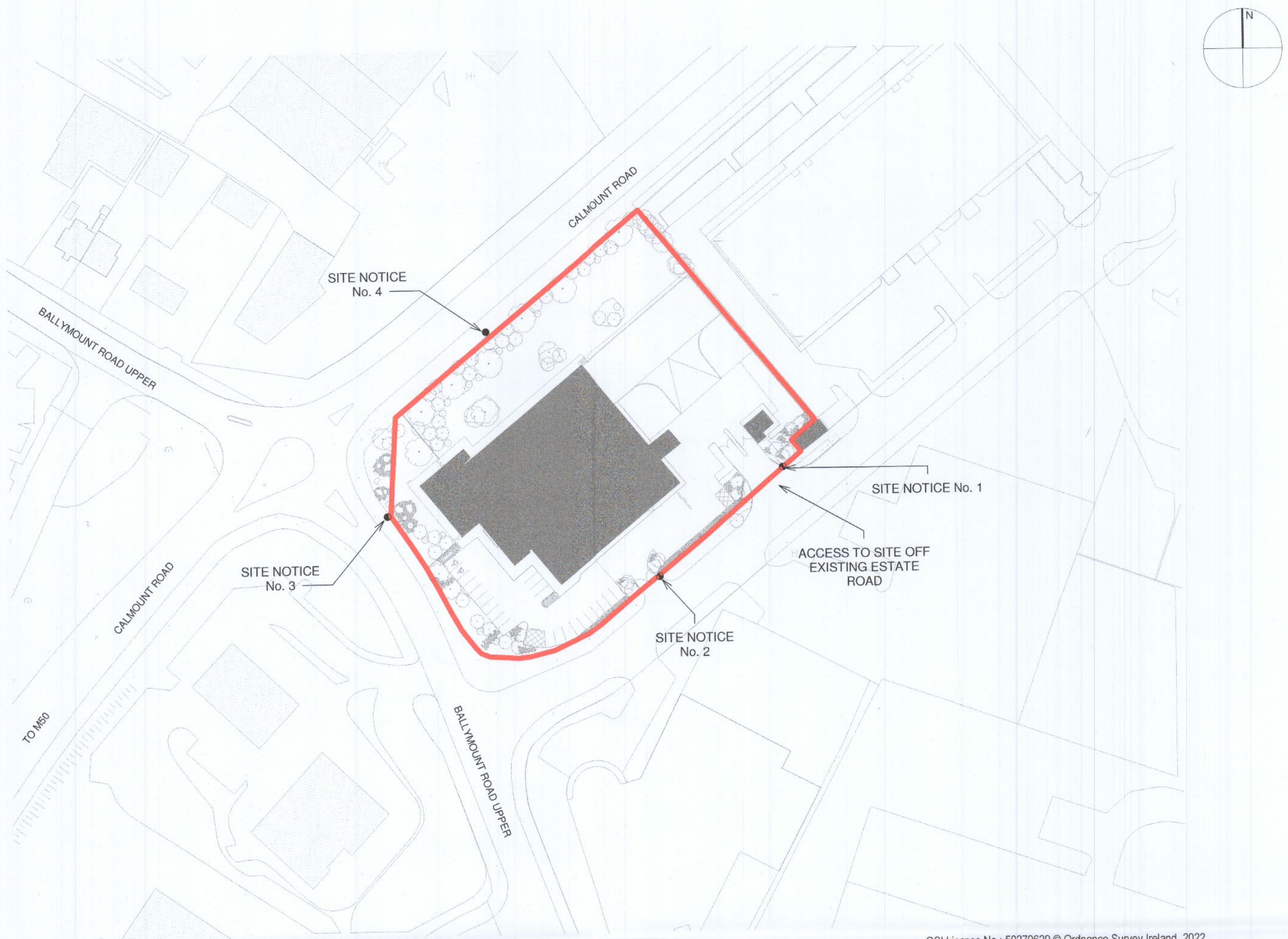
1 1001 Site Location Plan 1 : 1000
