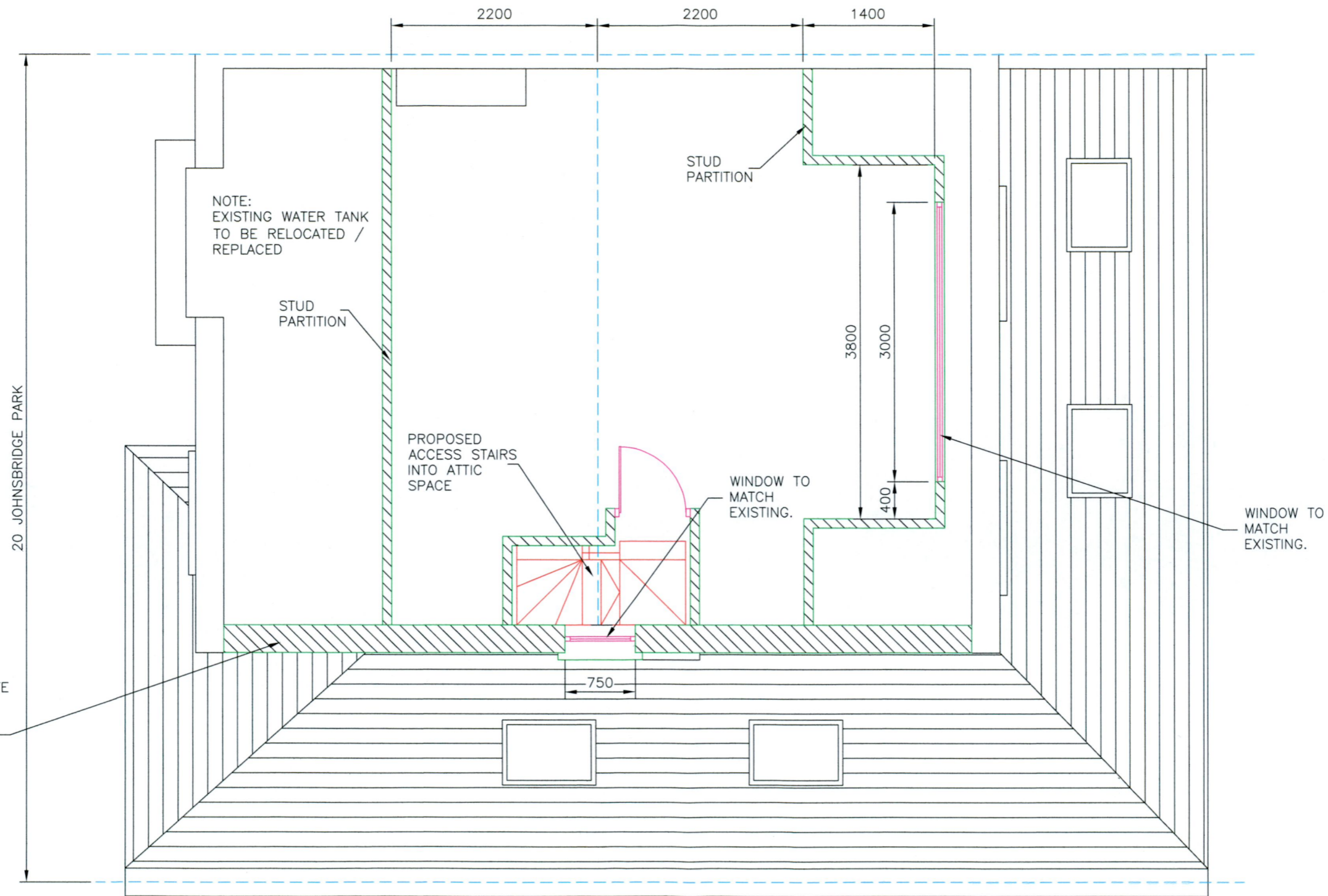
PROPOSED ATTIC FLOOR PLAN VIEW
