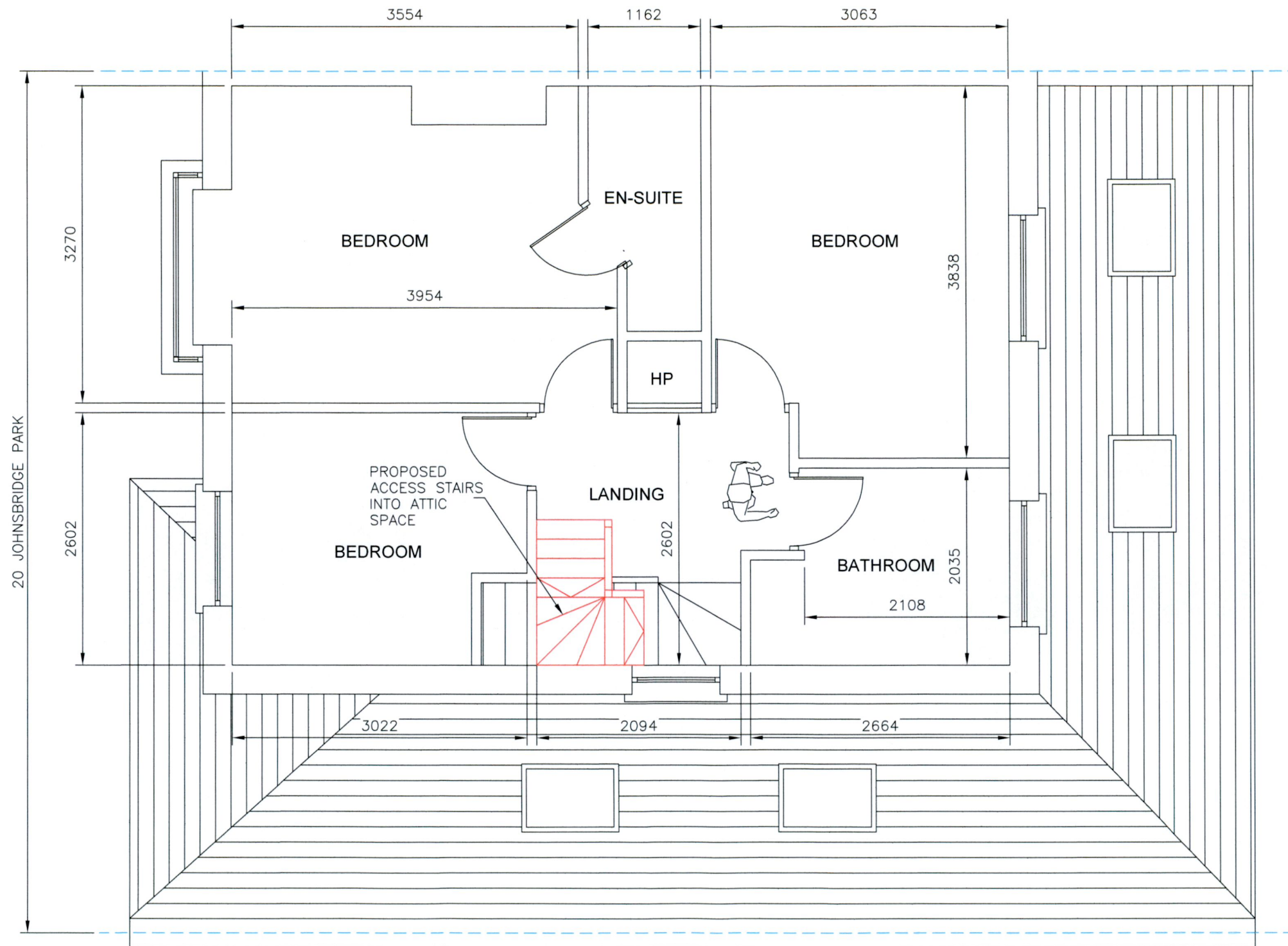
PROPOSED FIRST FLOOR PLAN VIEW
