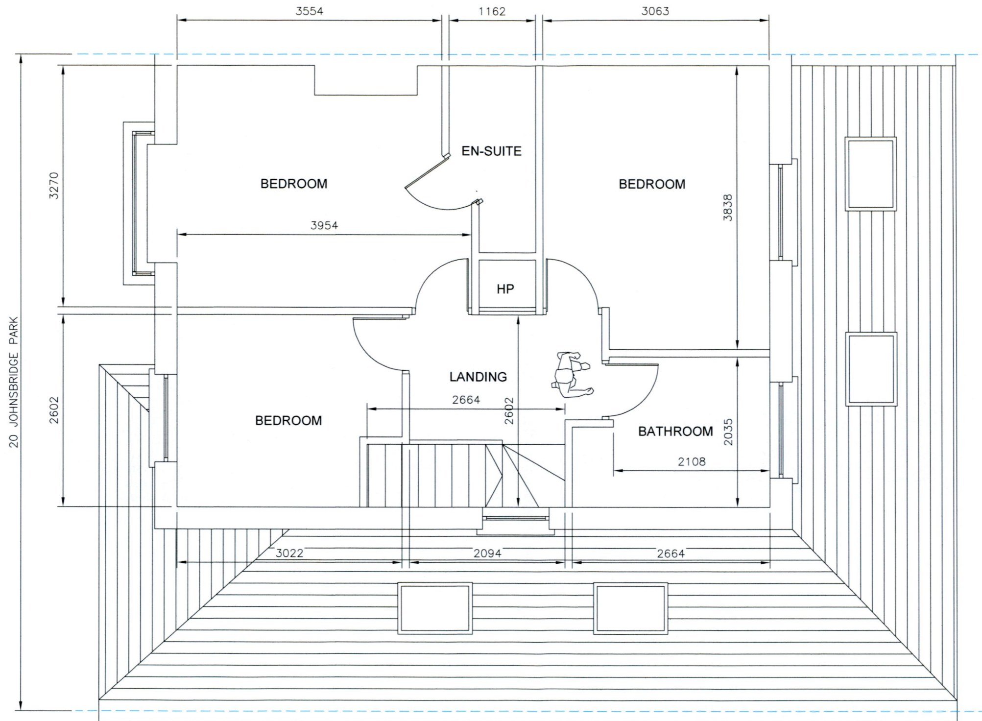
EXISTING FIRST FLOOR PLAN VIEW
