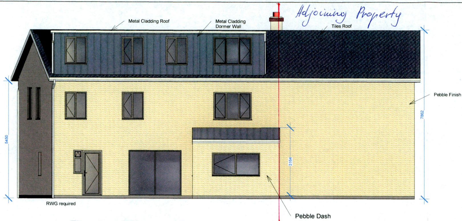
Rear Elevation
