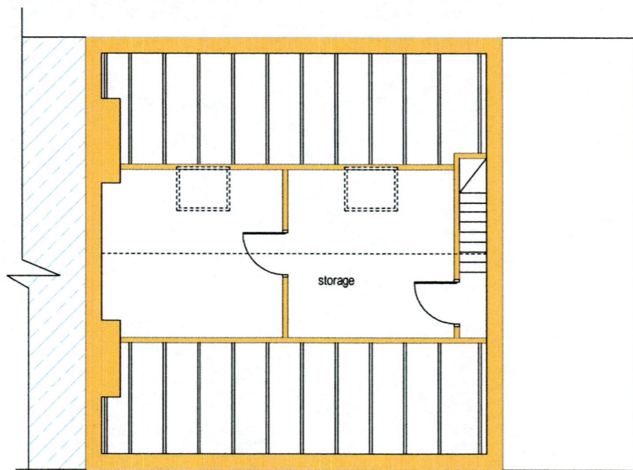
EXISTING ATTIC PLAN
