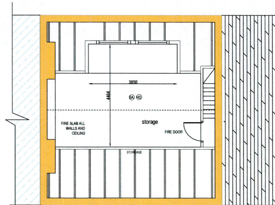
PROPOSED ATTIC PLAN
