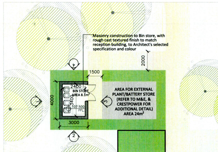
01 FLOOR PLAN PA-500 1:200
