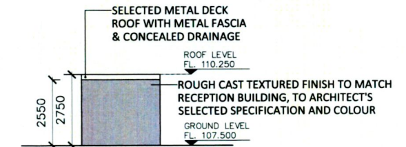
05 ELEVATION 02 PA500 1:200
