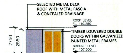
02 ELEVATION 03 PA500 1:200
