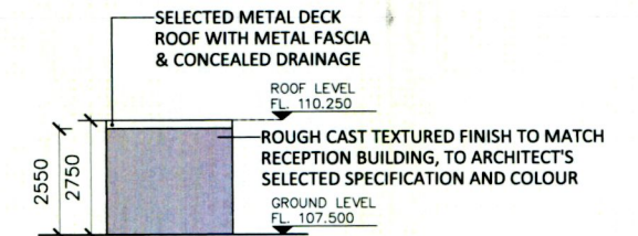
03 ELEVATION 04 PA500 1:200
