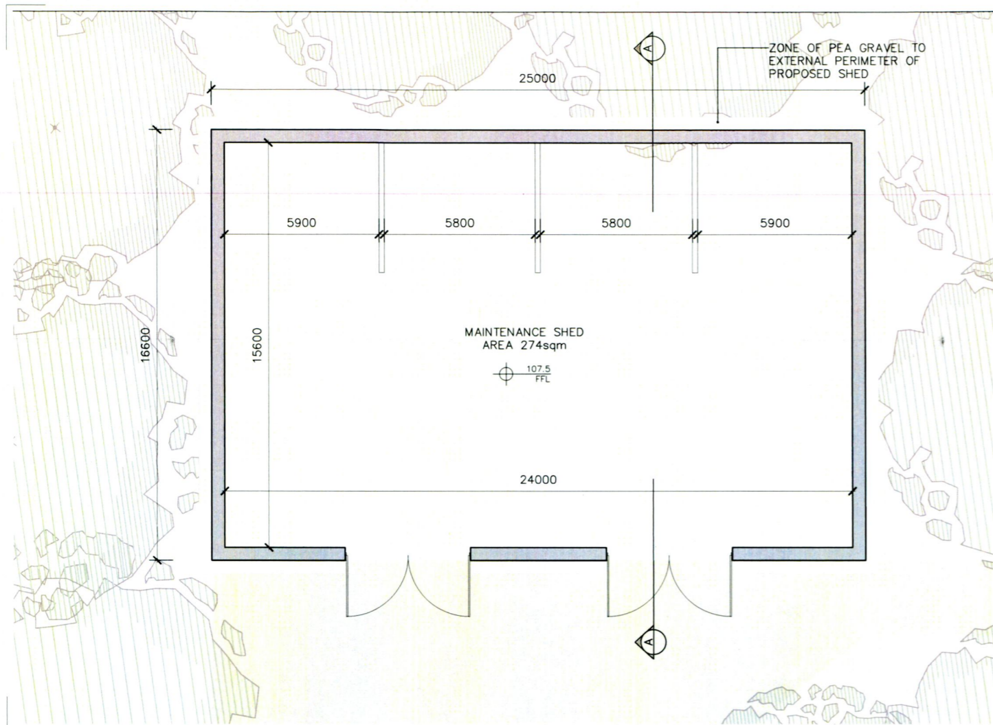
01 PROPOSED FLOOR PLAN PA-102 1:200
