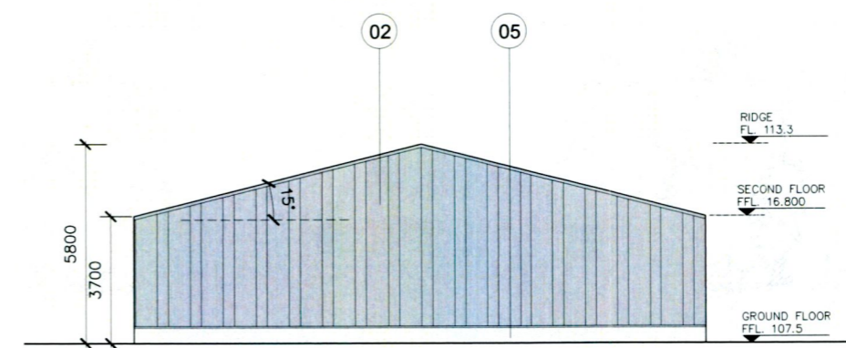
03 PROPOSED EAST ELEVATION PA-102 1:200
