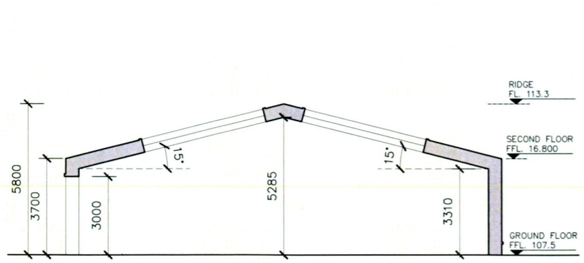
04 PROPOSED EAST ELEVATION PA-102 1:200
