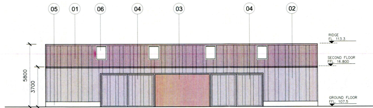
02 PROPOSED SOUTH ELEVATION PA-102 1:200
