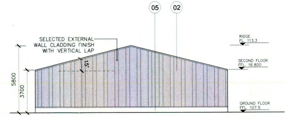
06 PROPOSED WEST ELEVATION PA-102 1:200
