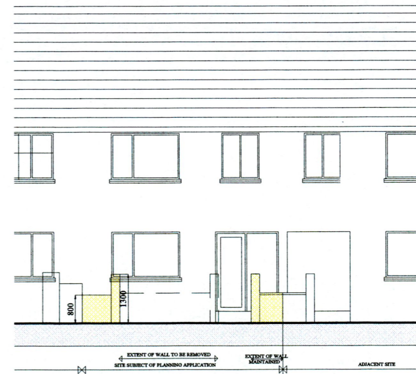
Front Elevation of House
