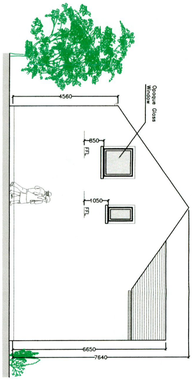
SIDE ELEVATION 1:100
