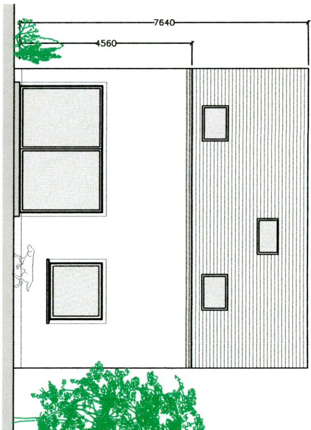
REAR ELEVATION 1:100
