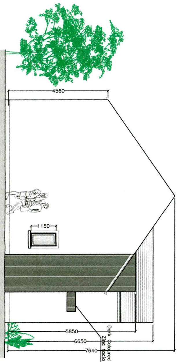
SIDE ELEVATION 1:100
