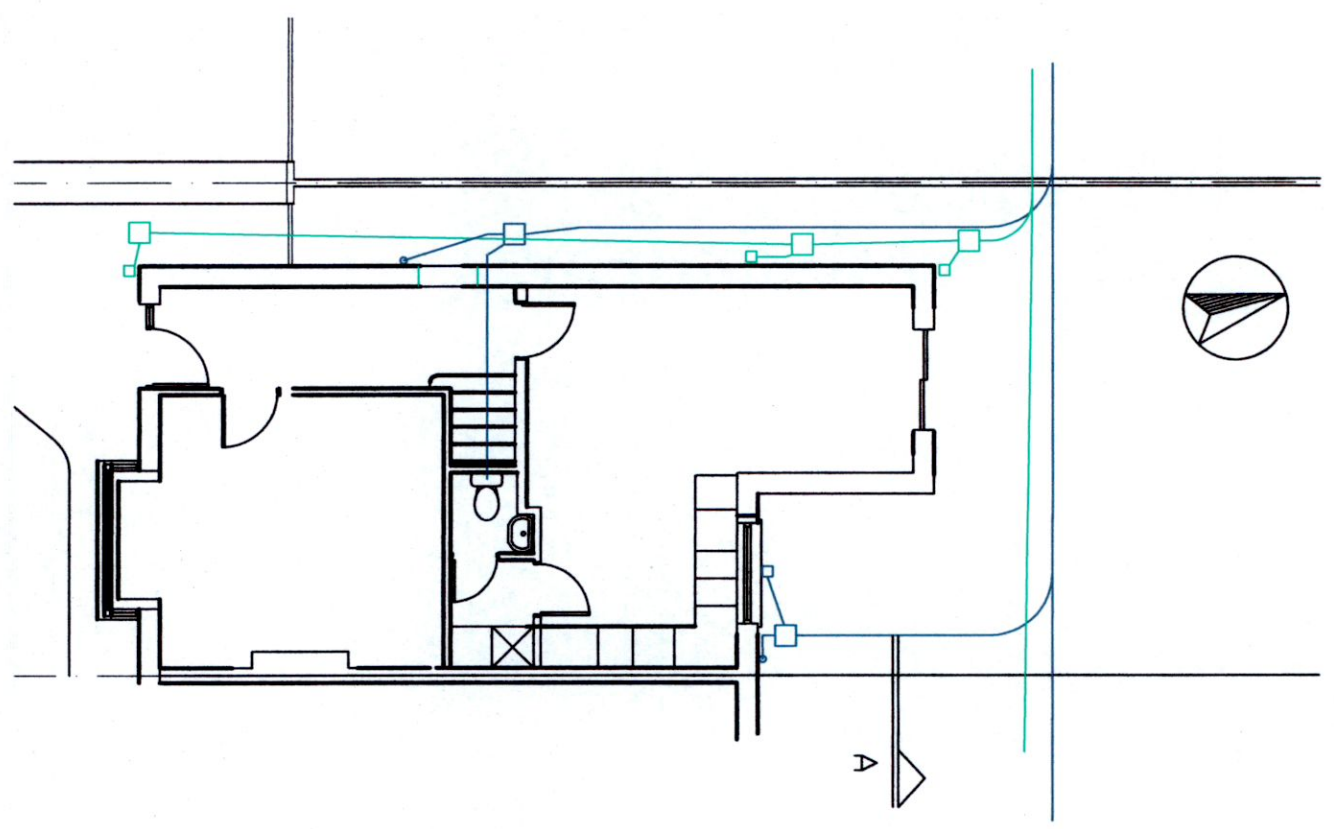
EXISTING DRAINAGE PLAN
