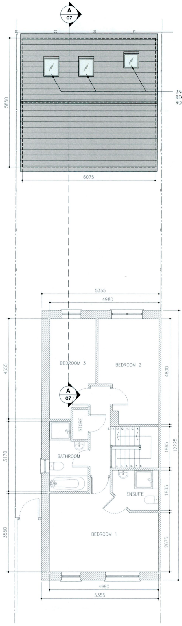
Proposed First Floor Layout SCALE 1:100 (TOTAL FLOOR AREA = 57.0sq.m)
