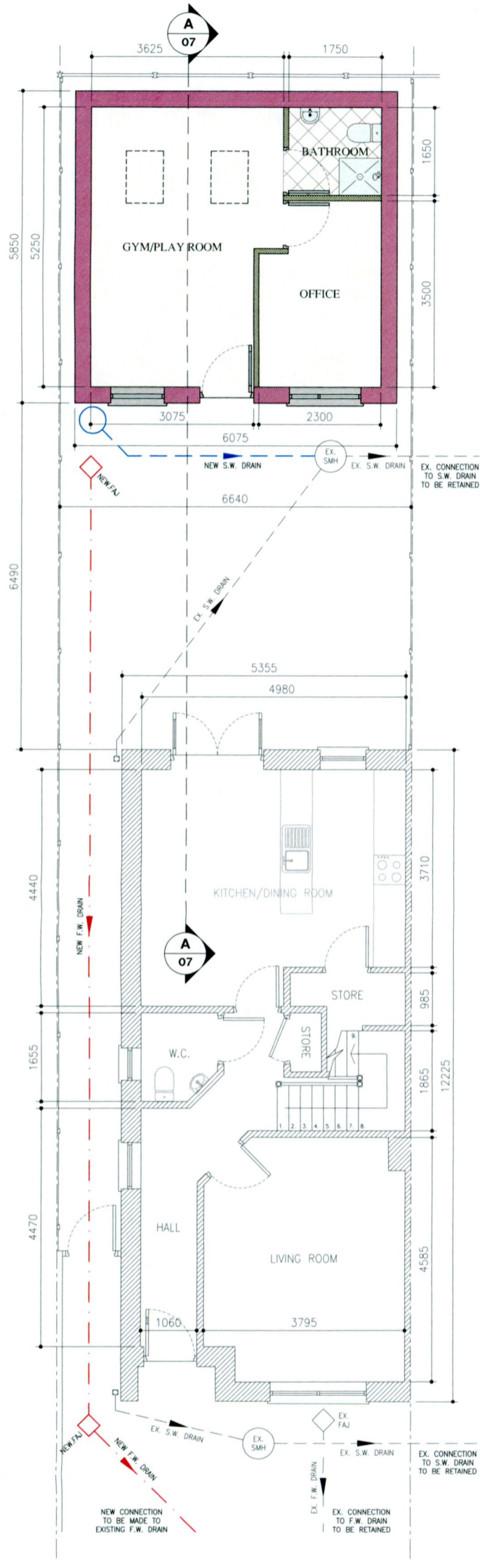
Proposed Ground Floor Layout SCALE 1:100 (TOTAL FLOOR AREA = 56.5sq.m) (TOTAL GARDEN BUILDING FLOOR AREA = 28.5sq.m)
