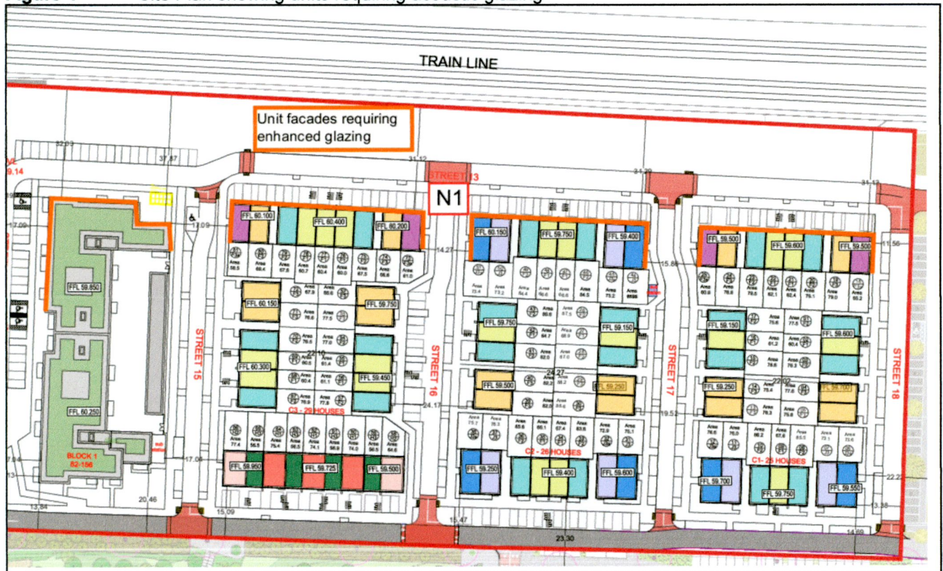
Figure 4 Site Plan showing units requiring acoustic glazing
