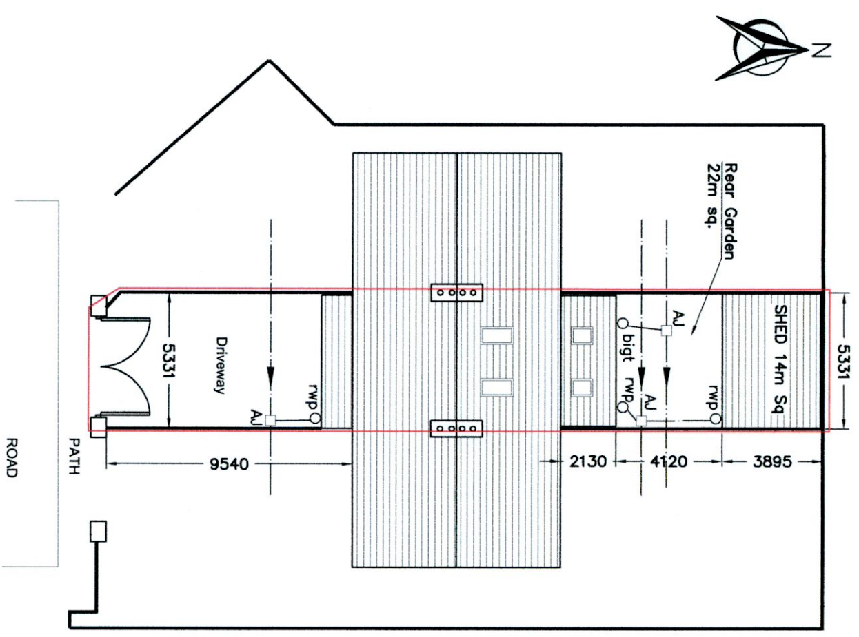
BLOCK PLAN & DRAINAGE LAYOUT SCALE 1:200
