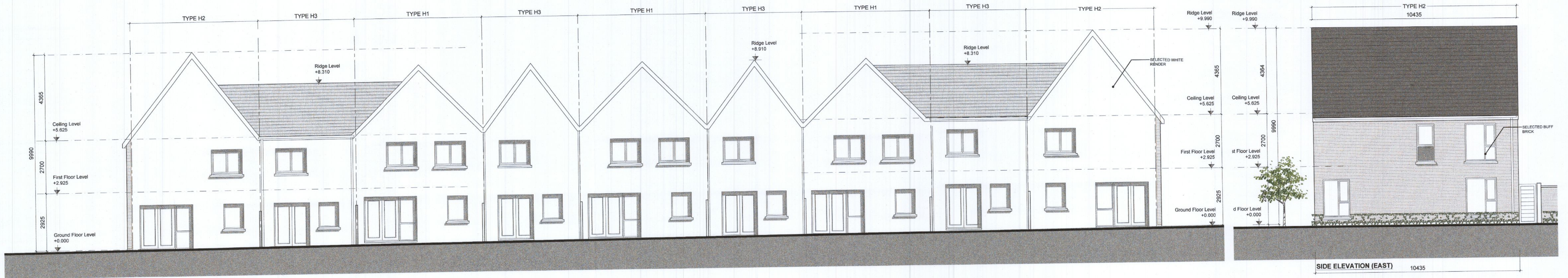
REAR ELEVATION
