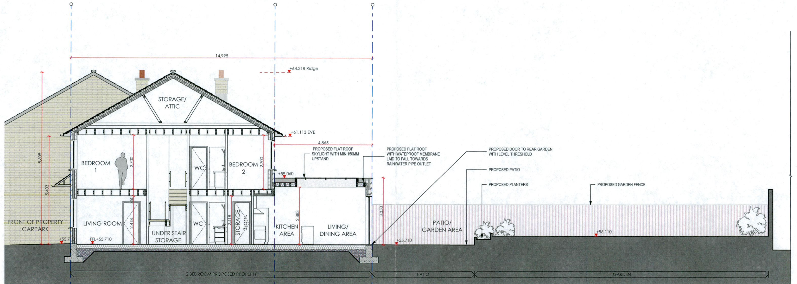
1 - PROPOSED NO.25A SECTION 1:100
