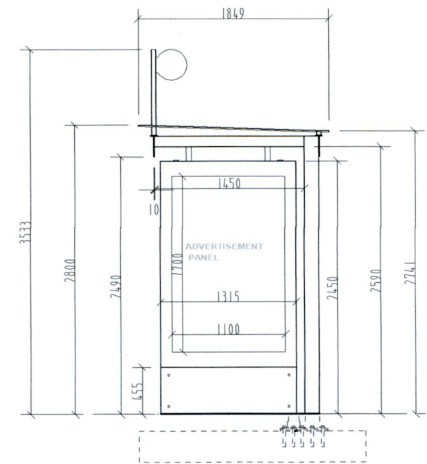
END ELEVATION ( Departure End )
