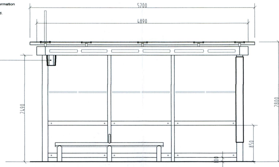
FRONT ELEVATION (ON SECTION LINE A - A')
