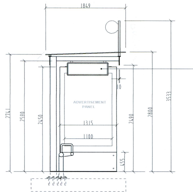
END ELEVATION ( Approach End )
