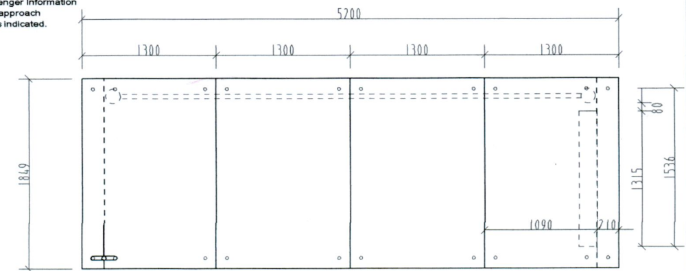
PLAN (SHOWING ROOF OVER)
