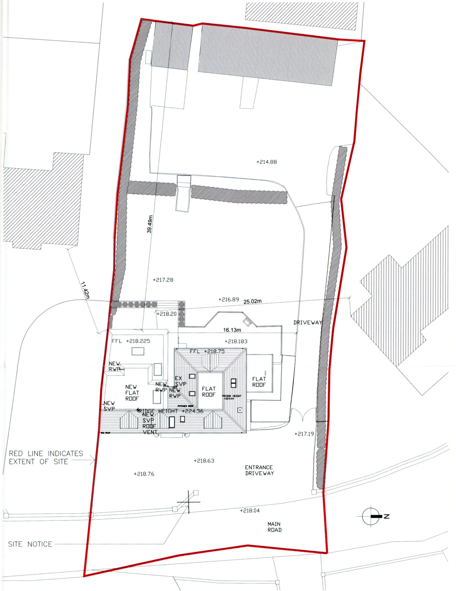
REVISED SITE LAYOUT PLAN SCALE 1 : 250
