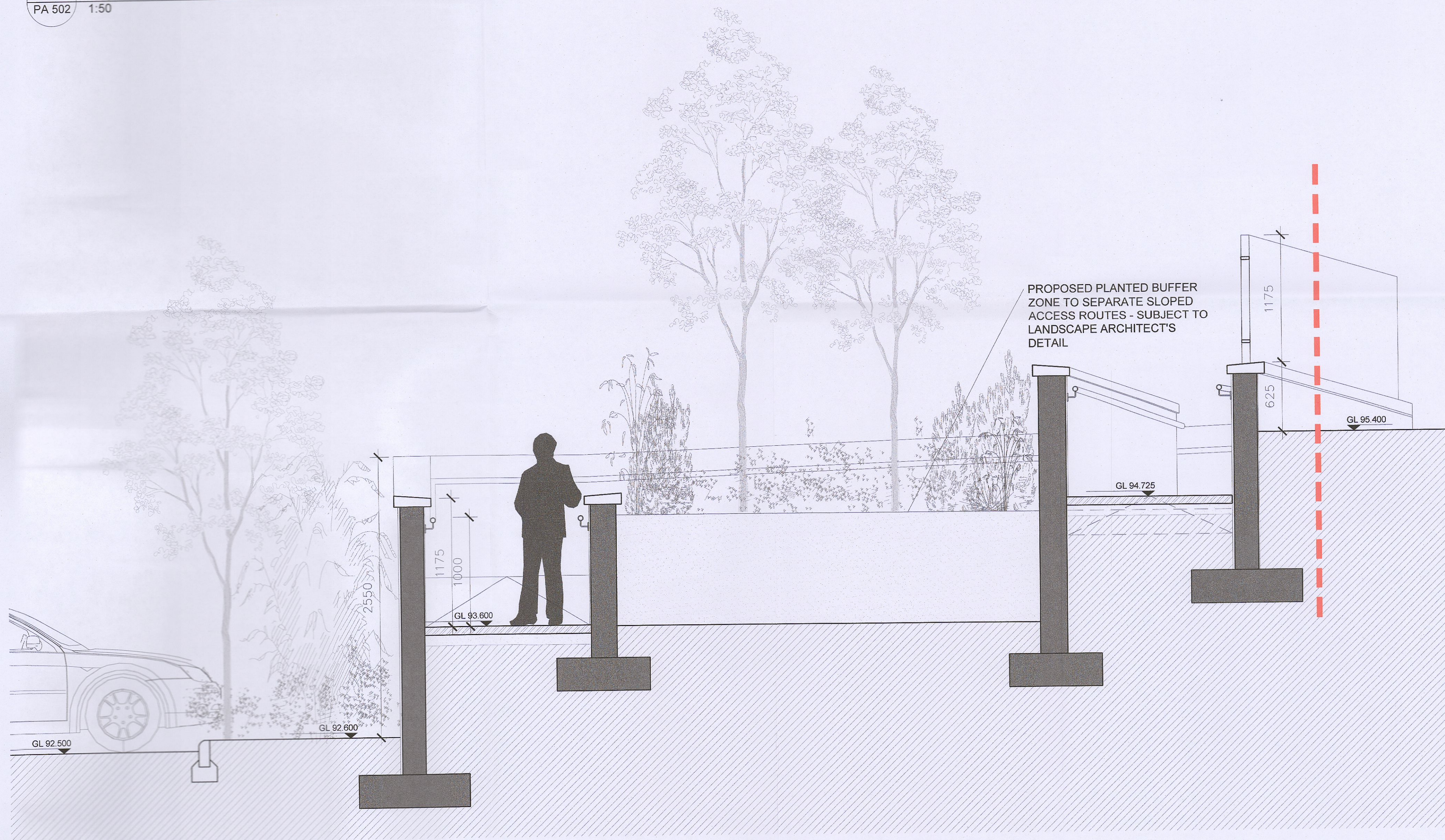
02 Proposed Boundary Wall (Boundaries I-J) Section PA 502 1:25
