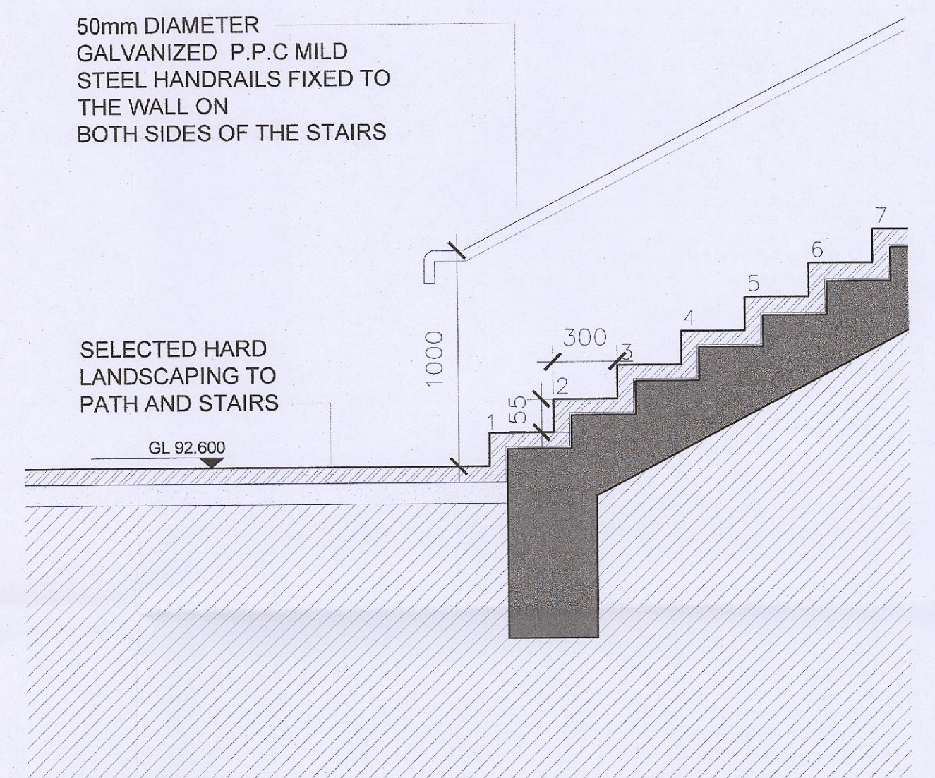
03 Proposed Stairs Section (Boundaries I-J) PA 502 1:25
