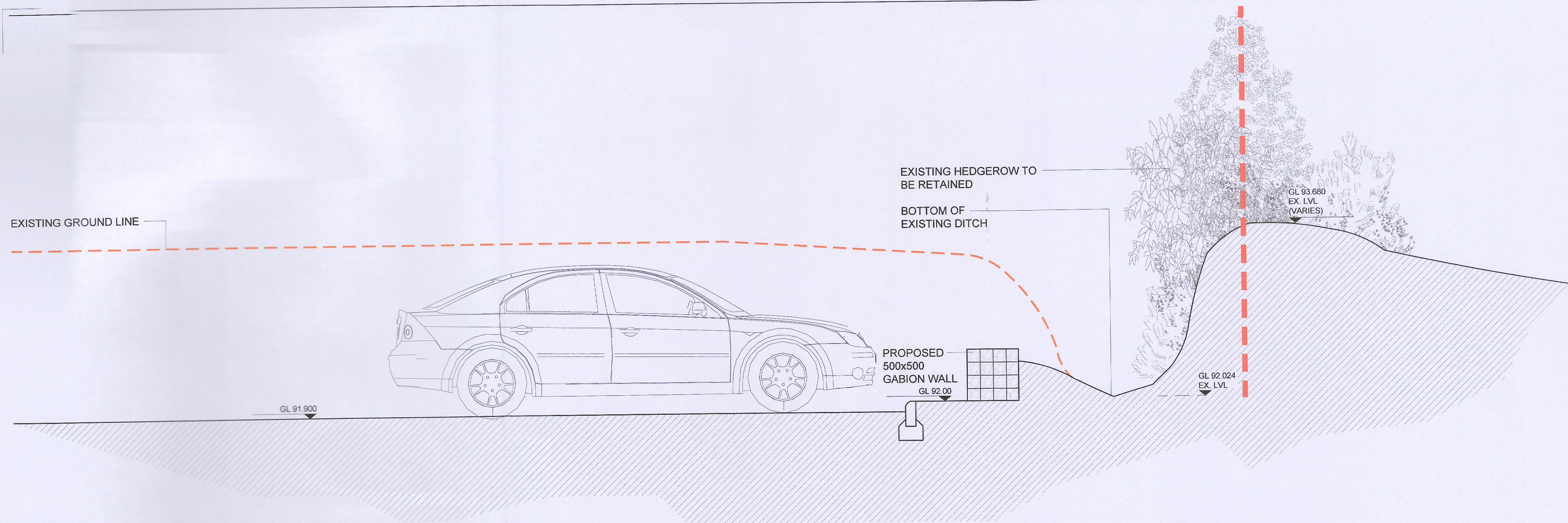
01 Proposed Boundary Wall (Boundaries D-E) Section PA 501 1:25
