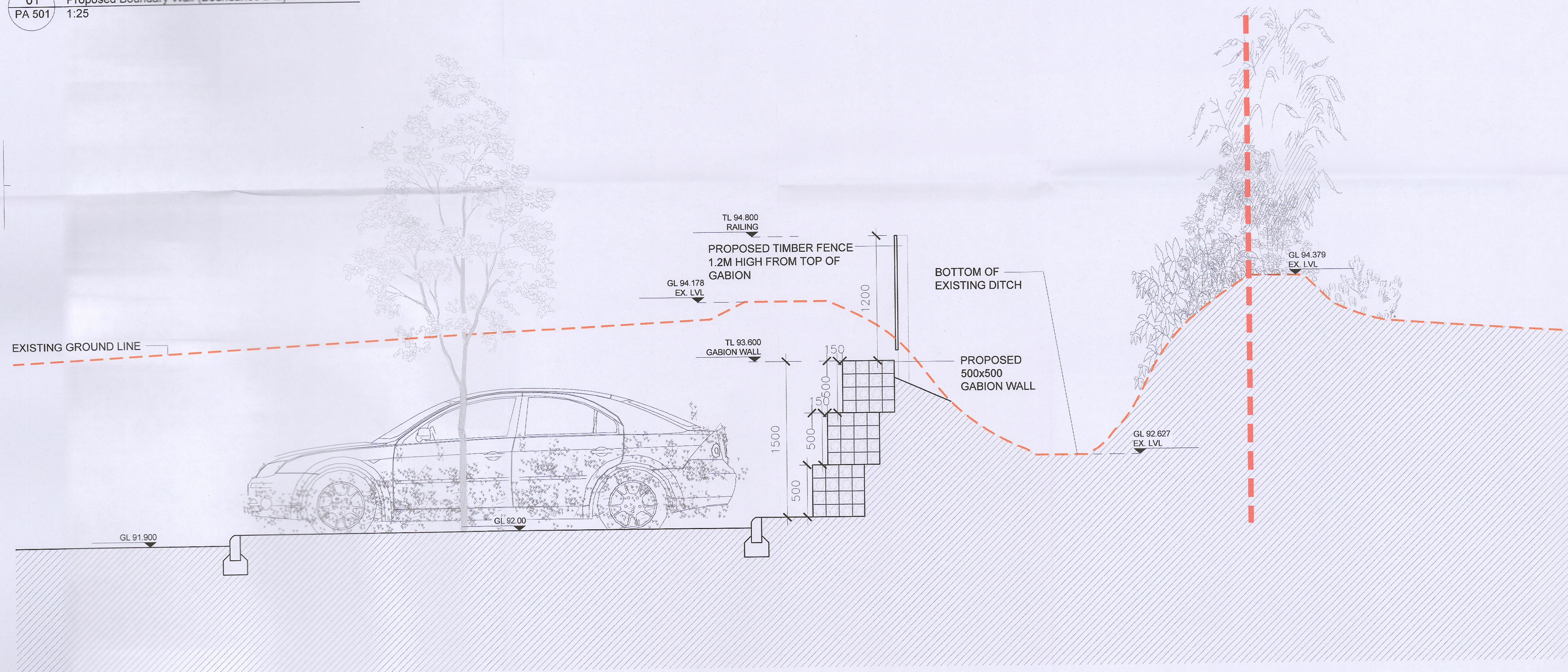
02 Proposed Boundary Wall (Boundaries D-E) Section PA 501 1:25
