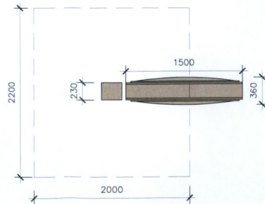
03 Proposed Flag Pole Plan PA-401 1:50
