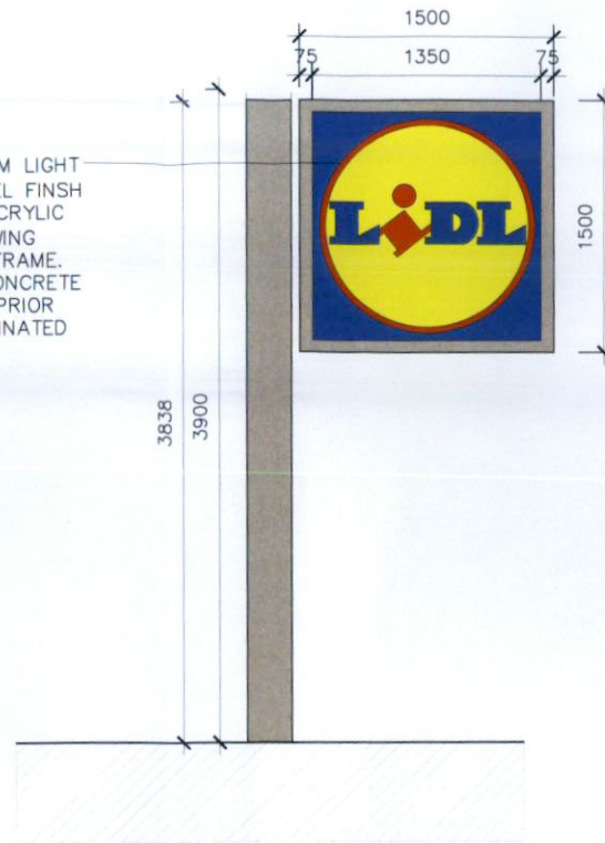
02 Proposed Flag Pole Front Elevation PA-401 1:50
