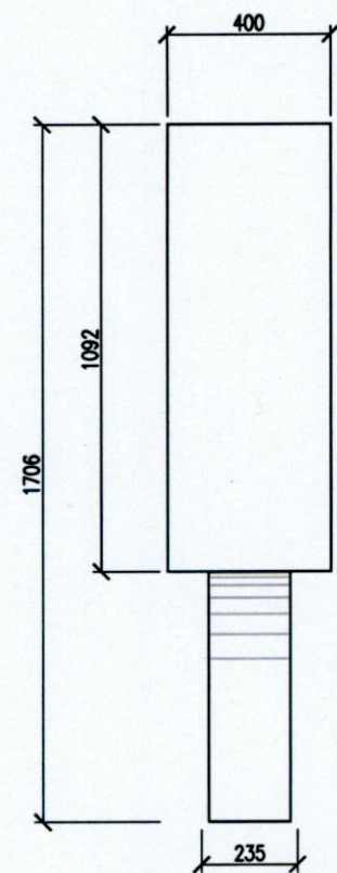
SIDE ELEVATION
