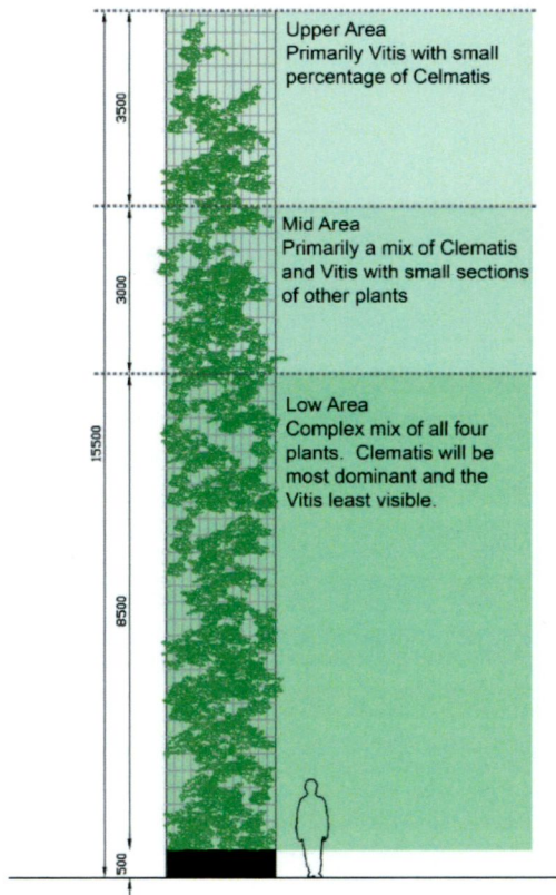
Fig 05 – Planting Species
