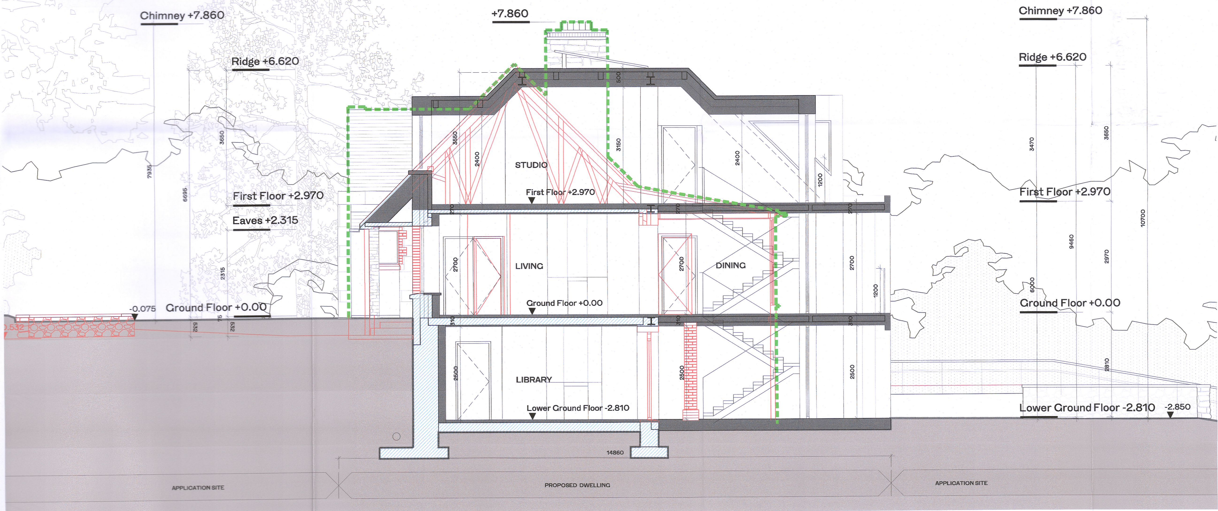
SECTION A-A - PROPOSED INTERVENTIONS - 1:50
