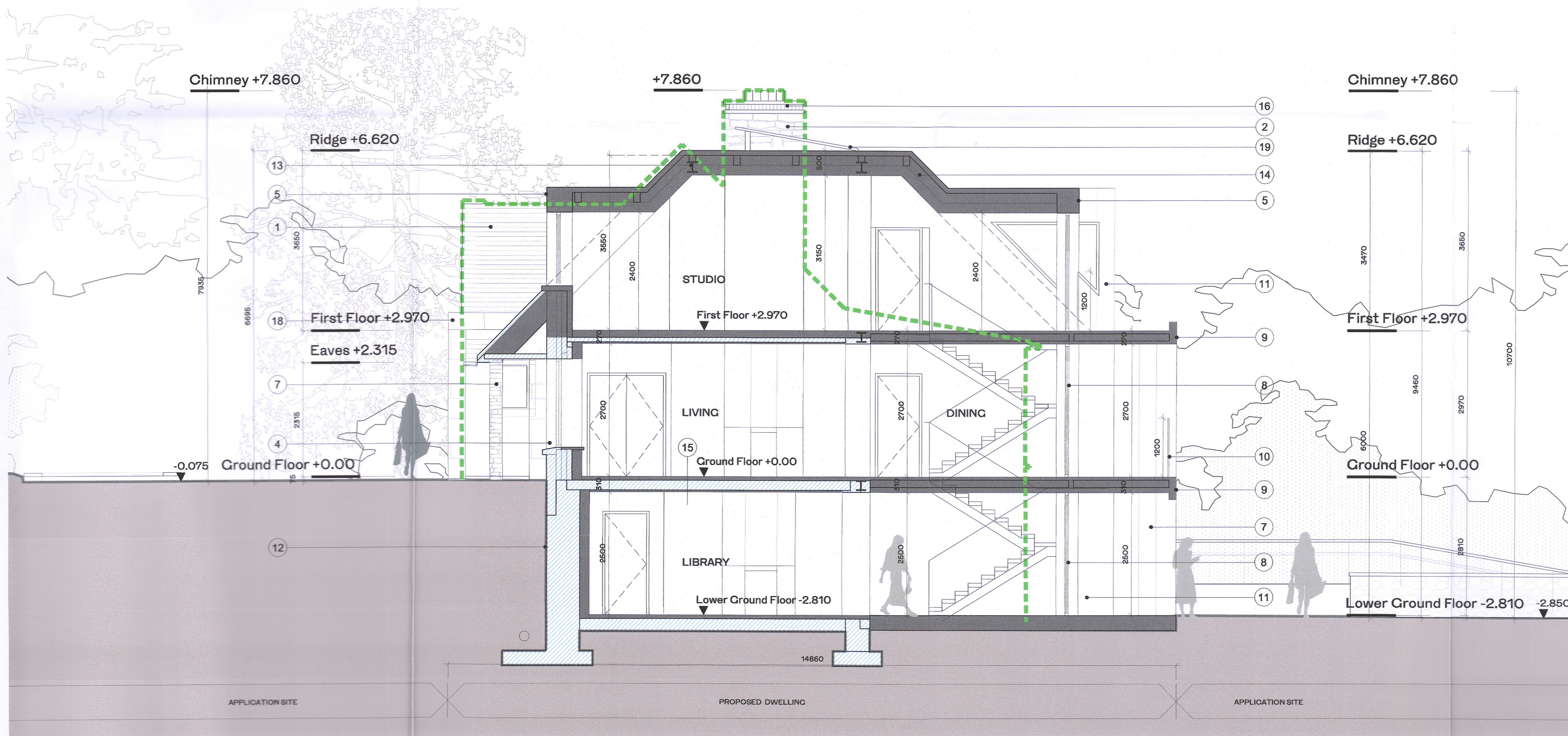
SECTION A-A - PROPOSED - 1:50
