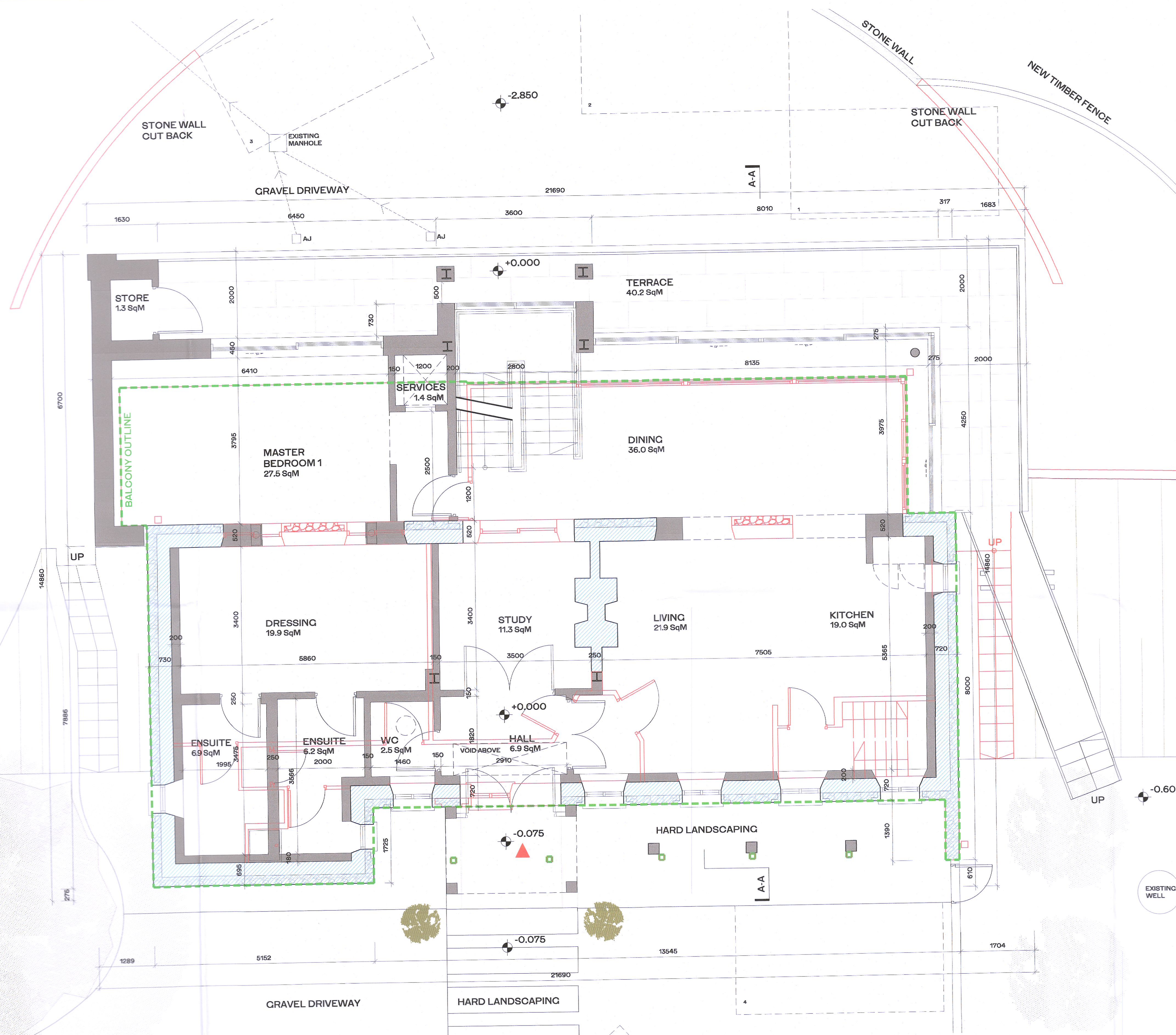
GROUND FLOOR PLAN - PROPOSED INTERVENTIONS
