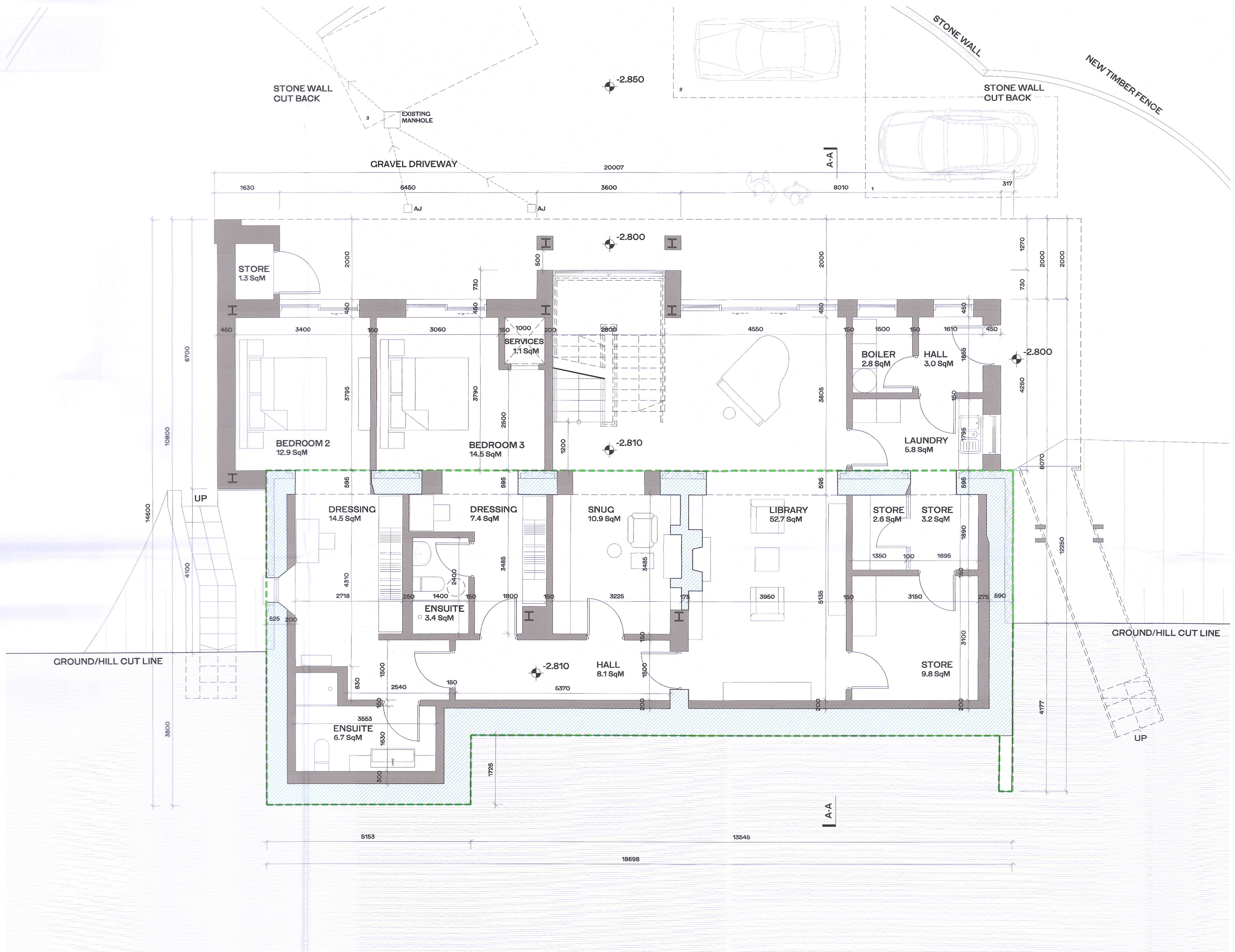
LOWER GROUND FLOOR PLAN - PROPOSED
