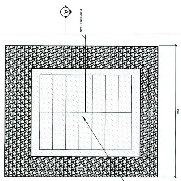
SAND POLISHING FILTER - PLAN SCALE 1:50 (A1)
