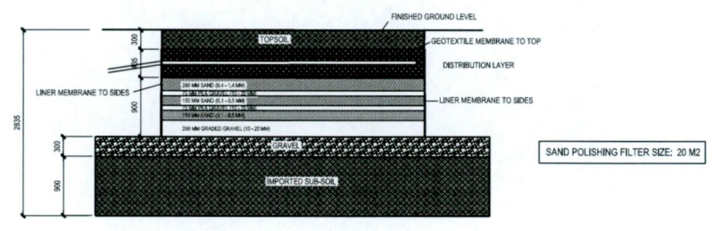
SAND POLISHING FILTER - SECTION SCALE 1:50 (A1)
