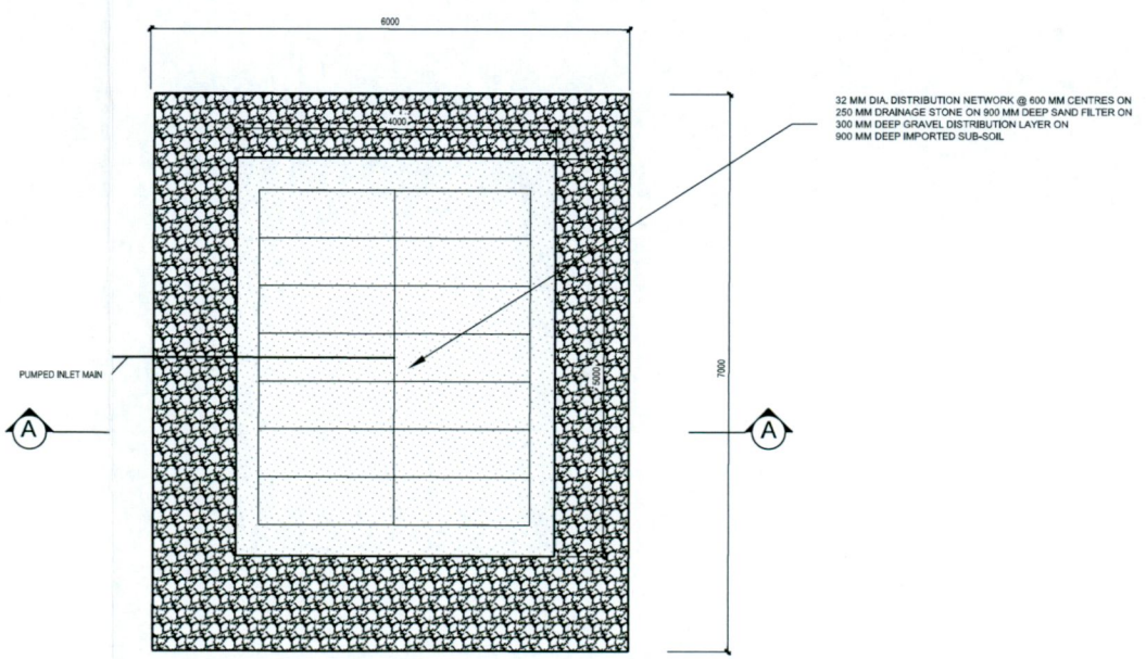
SAND POLISHING FILTER - PLAN SCALE 1:50 (A1)
