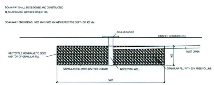
SURFACE WATER SOAKAWAY - SECTION SCALE 1:50 (A1)
