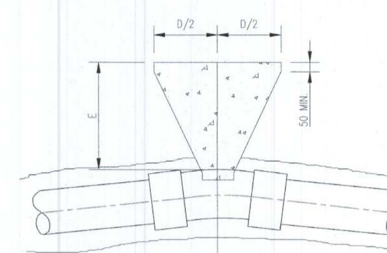
11.25° BEND
