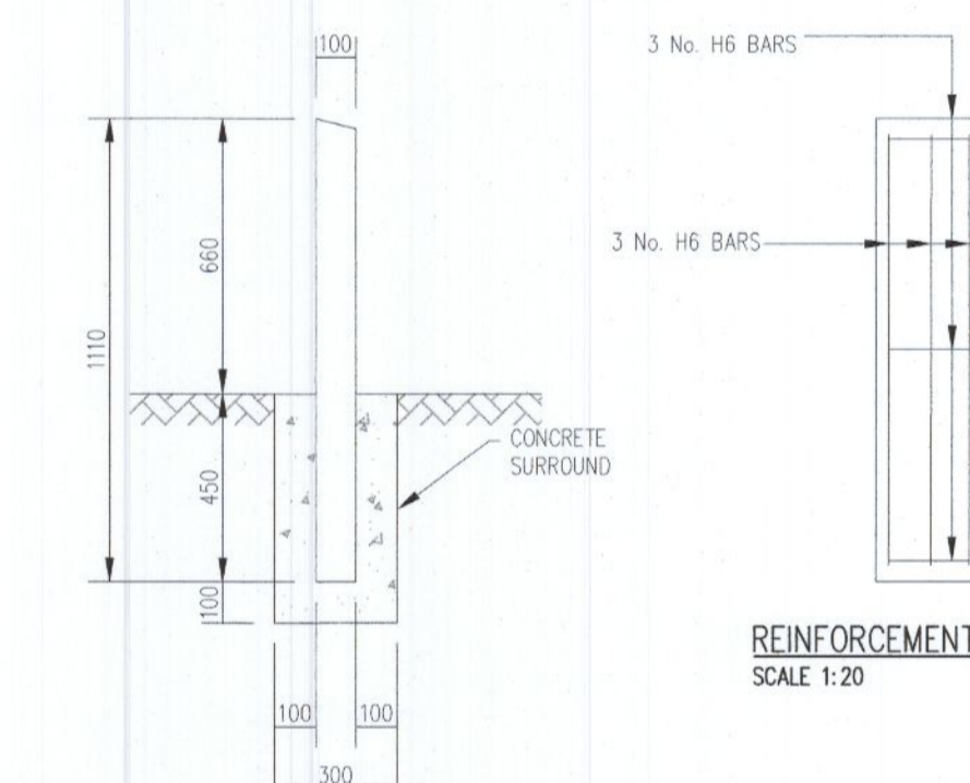
SECTION SCALE 1:20
