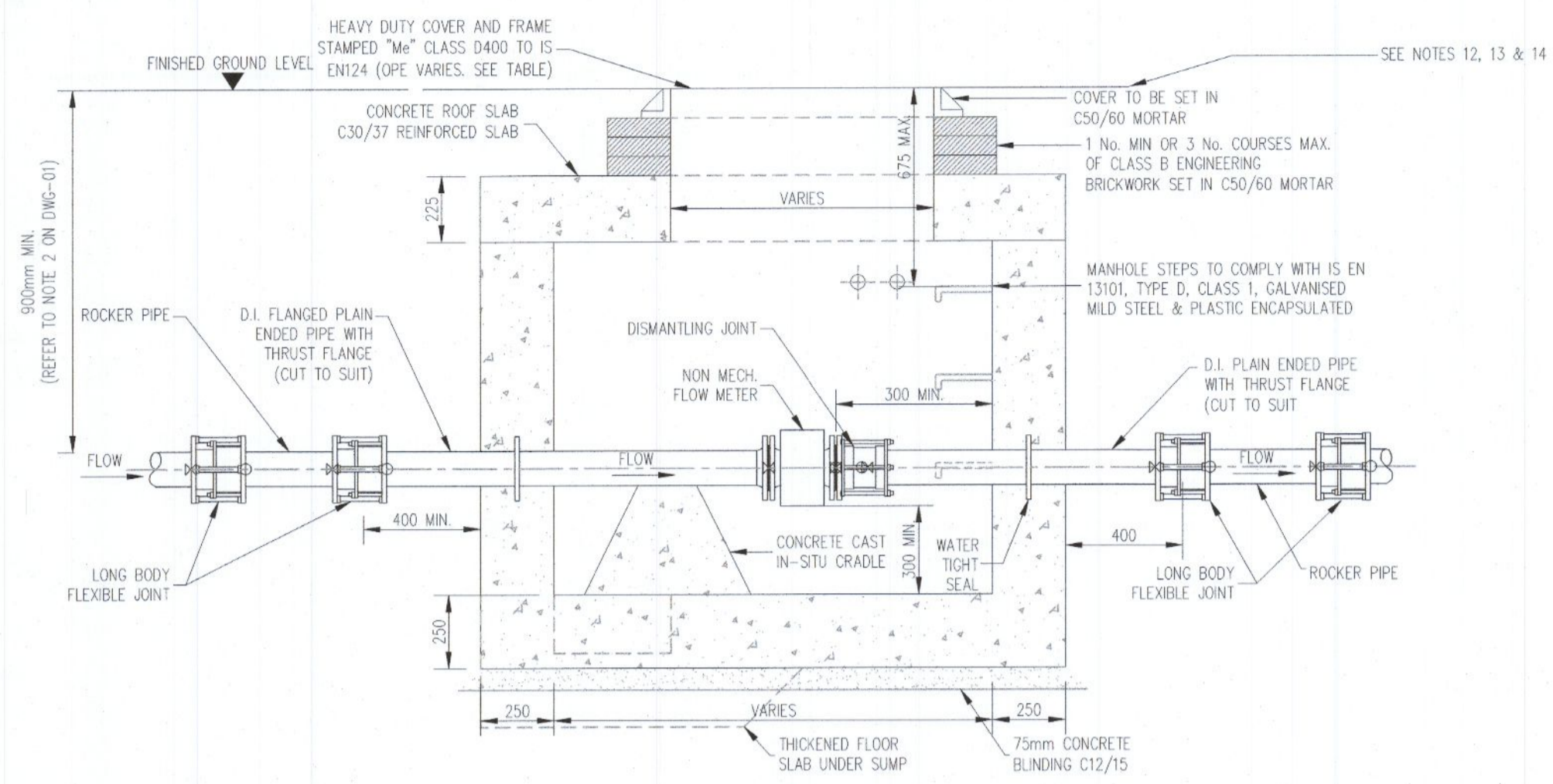
SECTION SCALE 1:20
