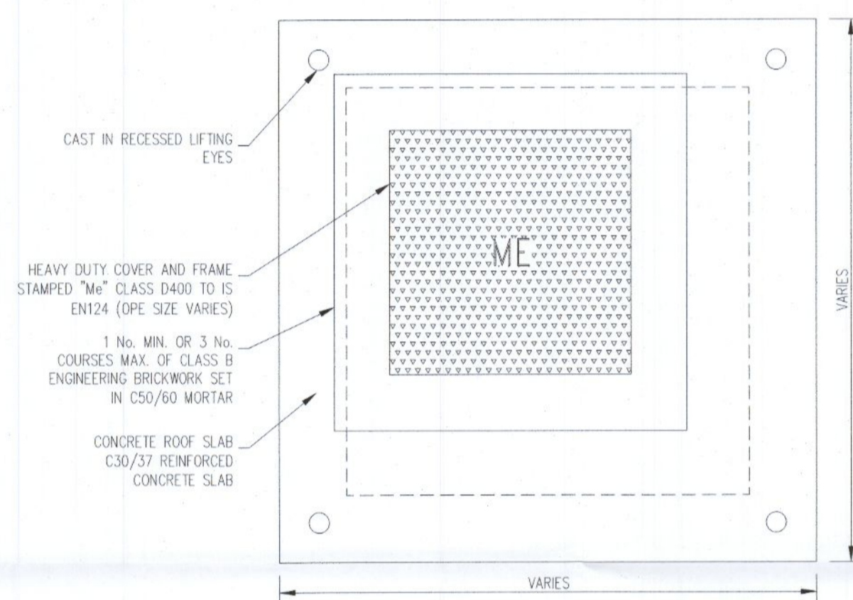
ROOF PLAN SCALE 1:20
