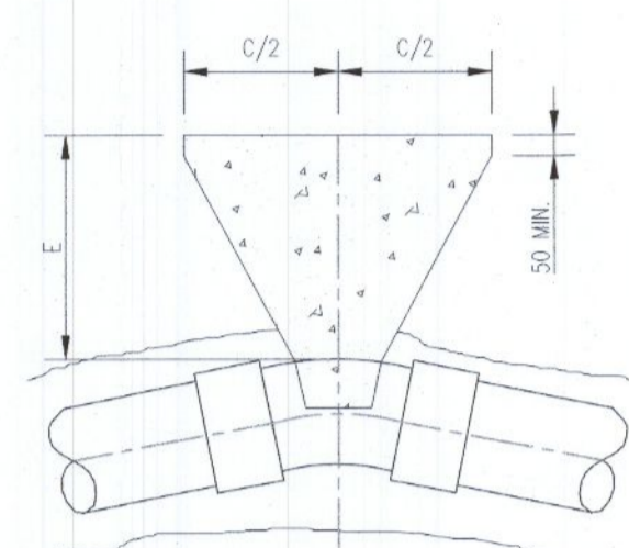
22.5° BEND
