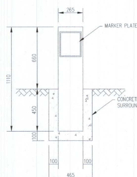
ELEVATION SCALE 1:20
