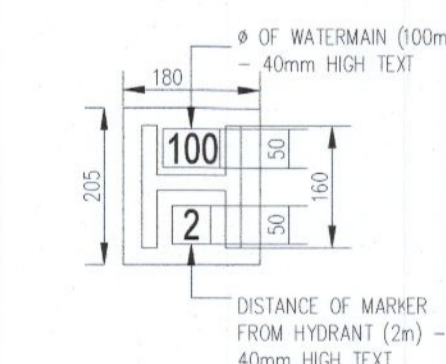
HYDRANT
