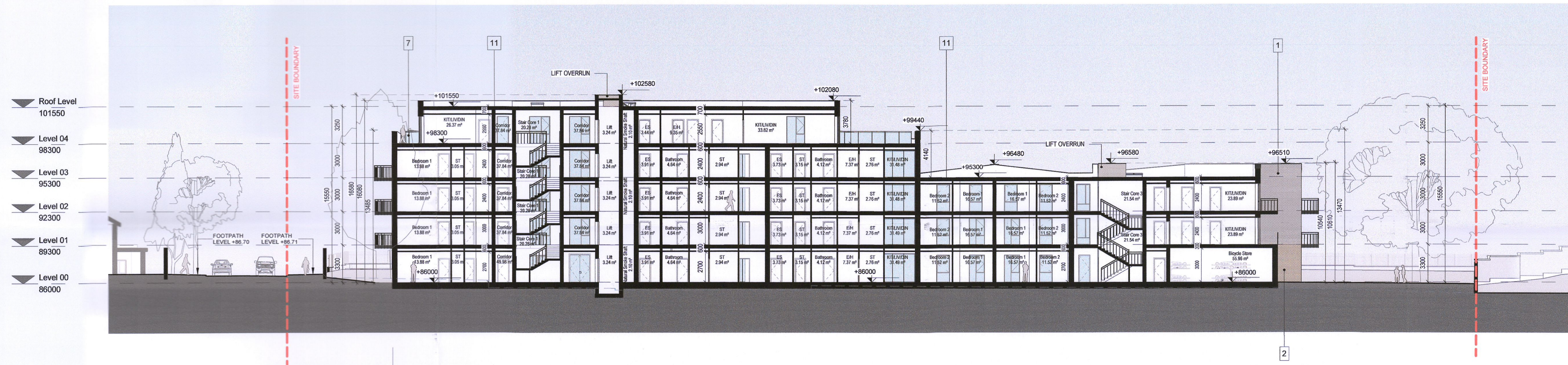
B-B PROPOSED SECTION B-B 1:200
