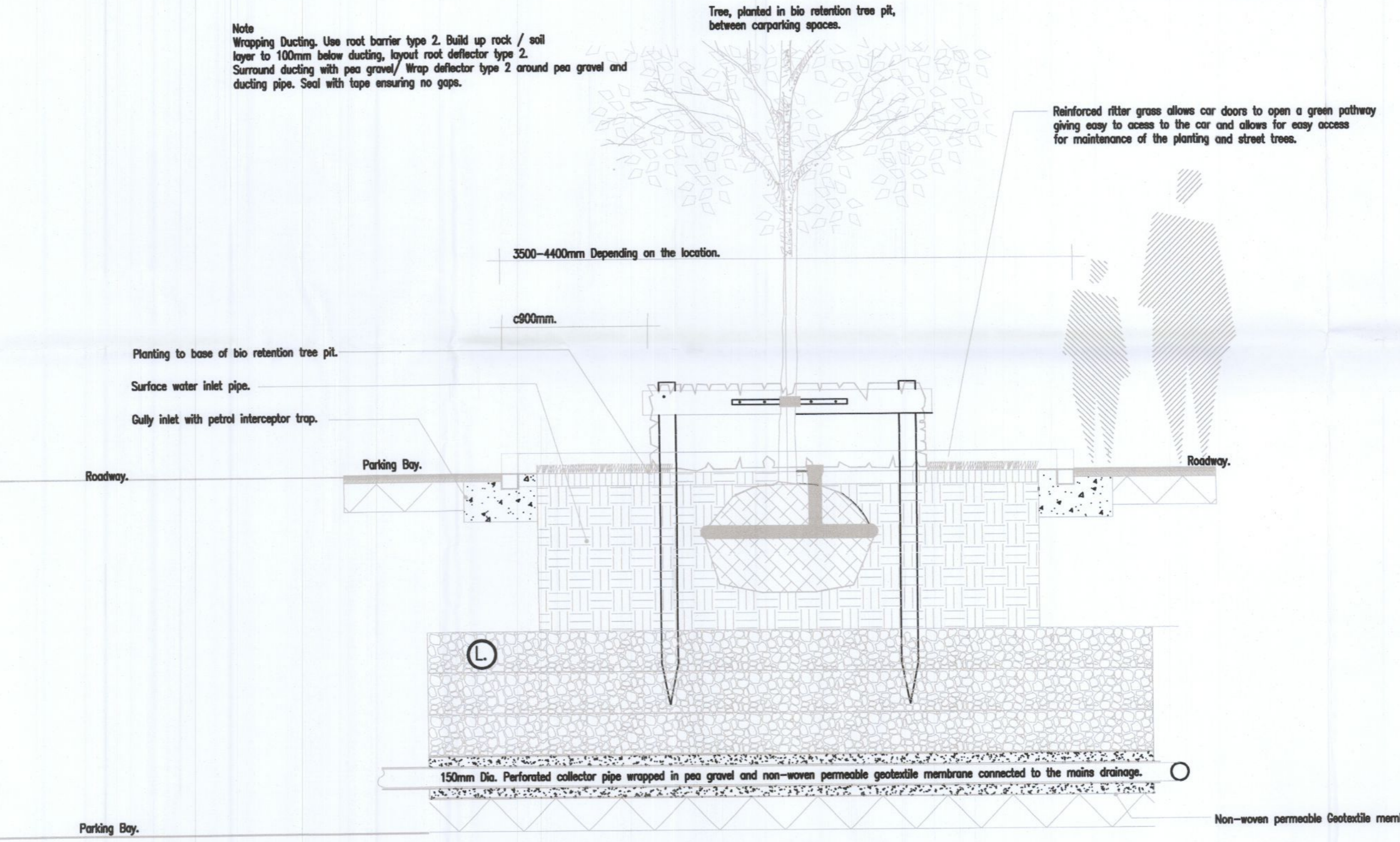
Section B-B Detail D01. Scale @ 1:25
