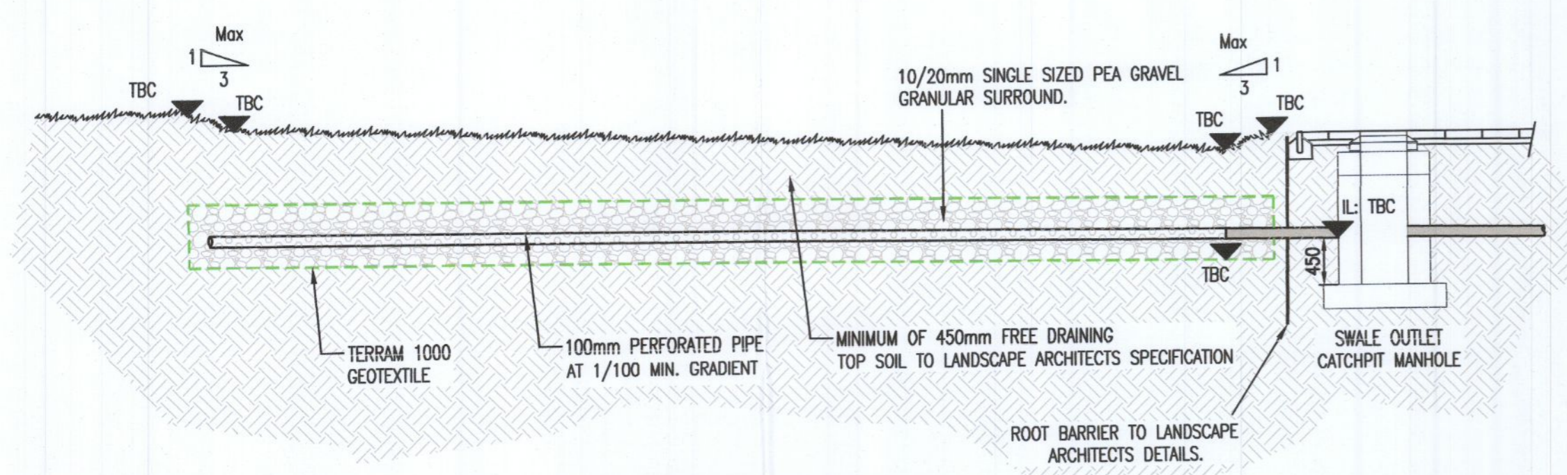
TYPICAL SWALE CROSS SECTION SCALE 1:50 @A1
