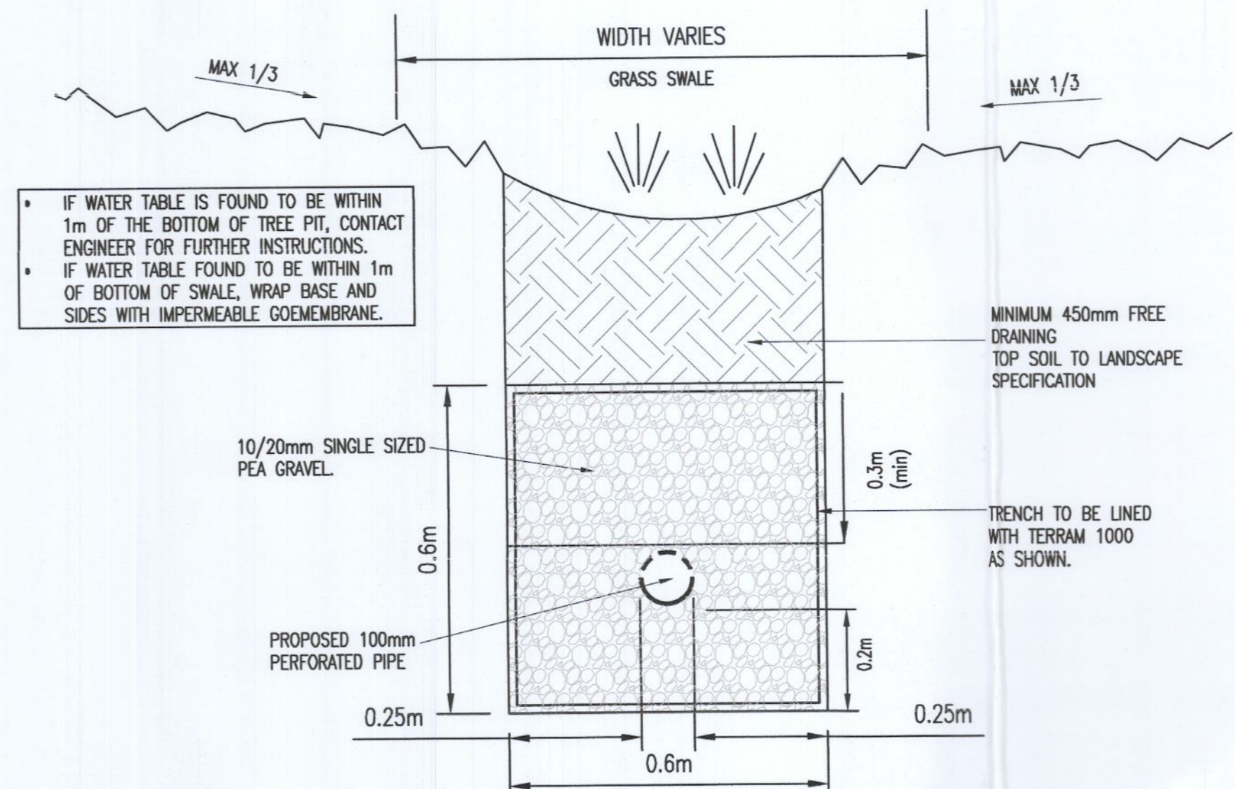
TYPICAL SECTION THROUGH PROPOSED SWALES SCALE 1:10 @A1
