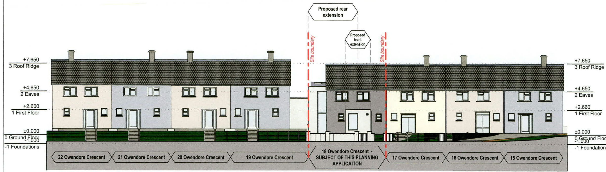
CONTEXTUAL ELEVATION
