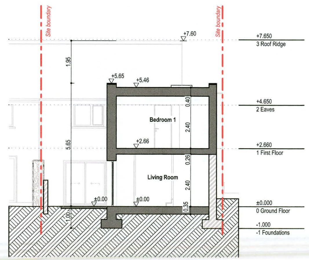
PROPOSED SECTION
