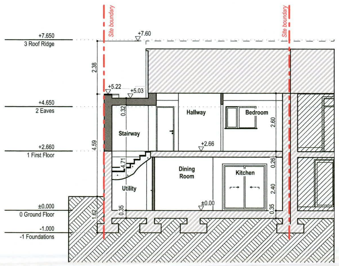
PROPOSED SECTION
