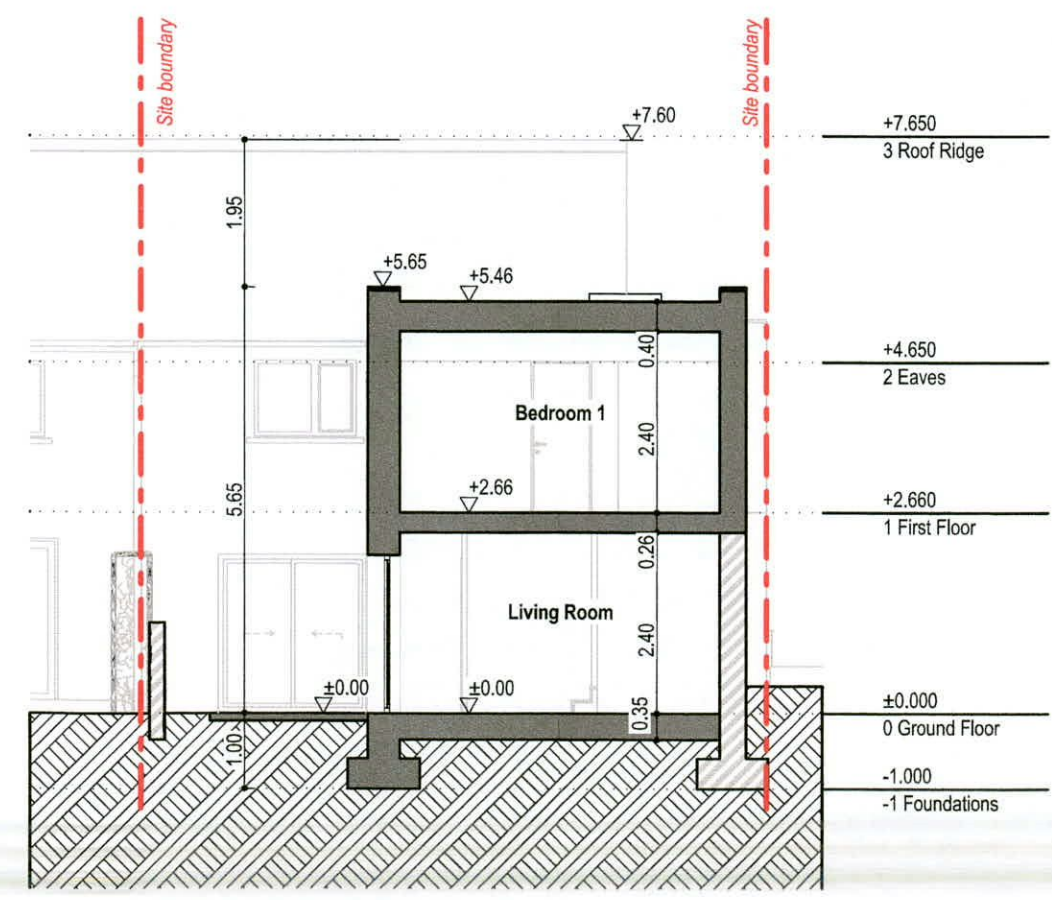
PROPOSED SECTION
