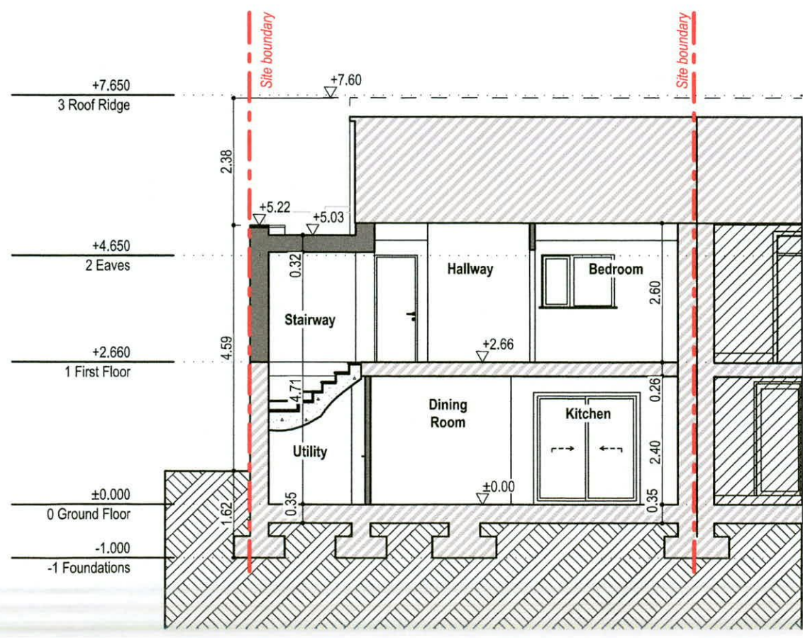
PROPOSED SECTION
