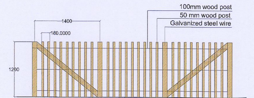
1.2m High Timber fence for Play Area sc 1/50
