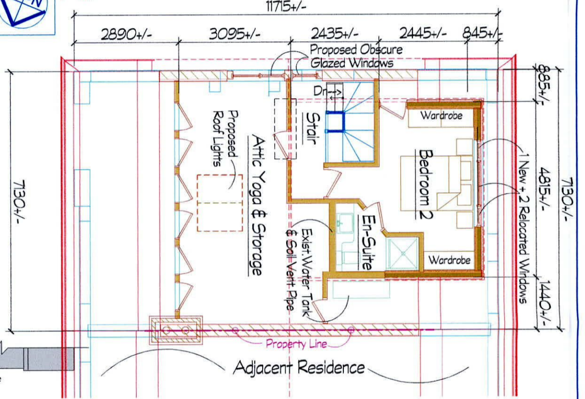
2 PROPOSED ATTIC FLOOR PLAN 1:100
