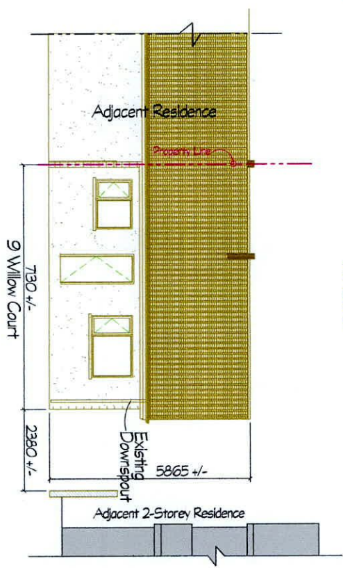
3 EXISTING FRONT (EAST) ELEVATION 1:150
