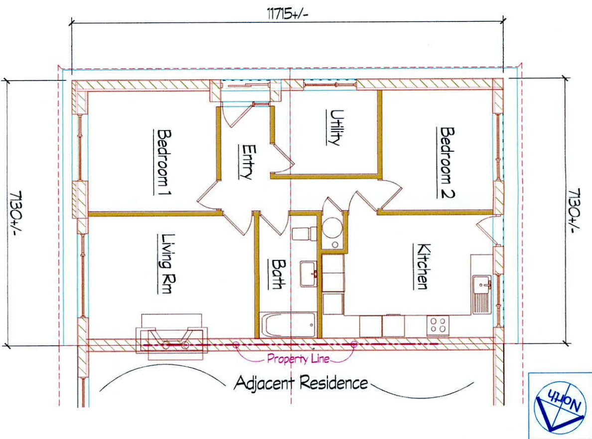
1 EXISTING GROUND FLOOR PLAN 1:100
