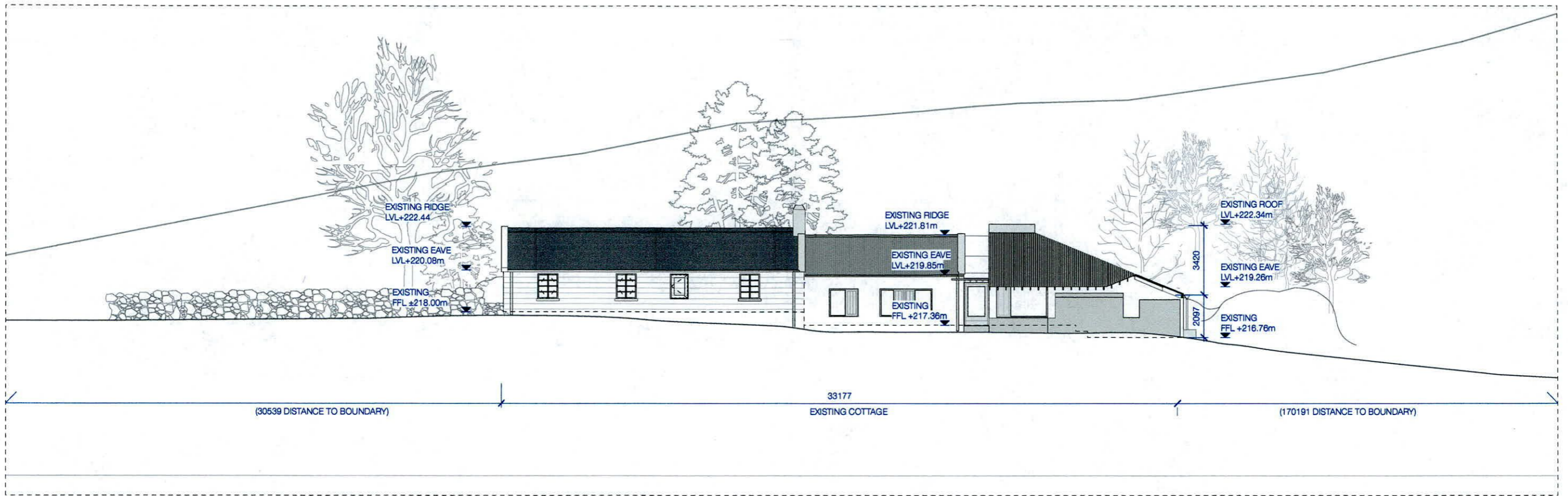
East (FRONT) Elevation - Existing SCALE 1: 200
