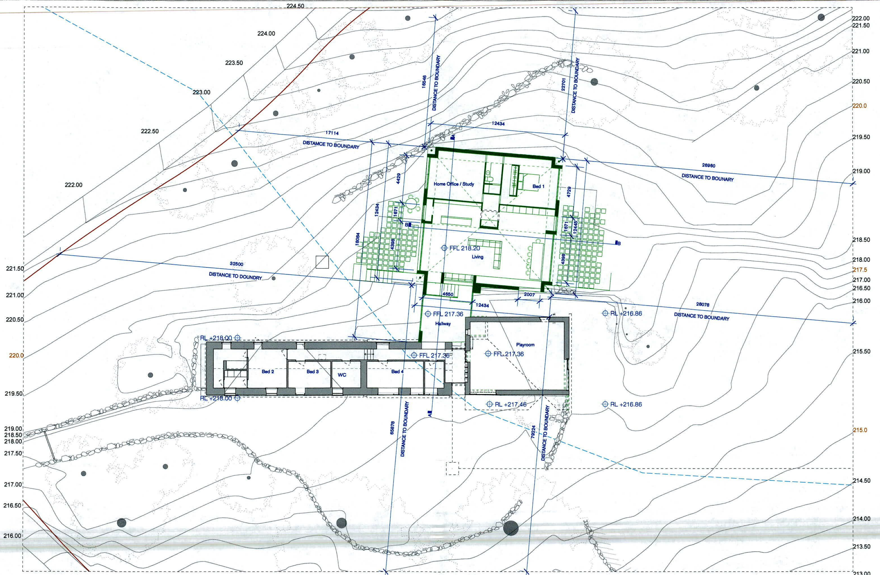
Ground Floor Plan - Proposed SCALE 1:200
