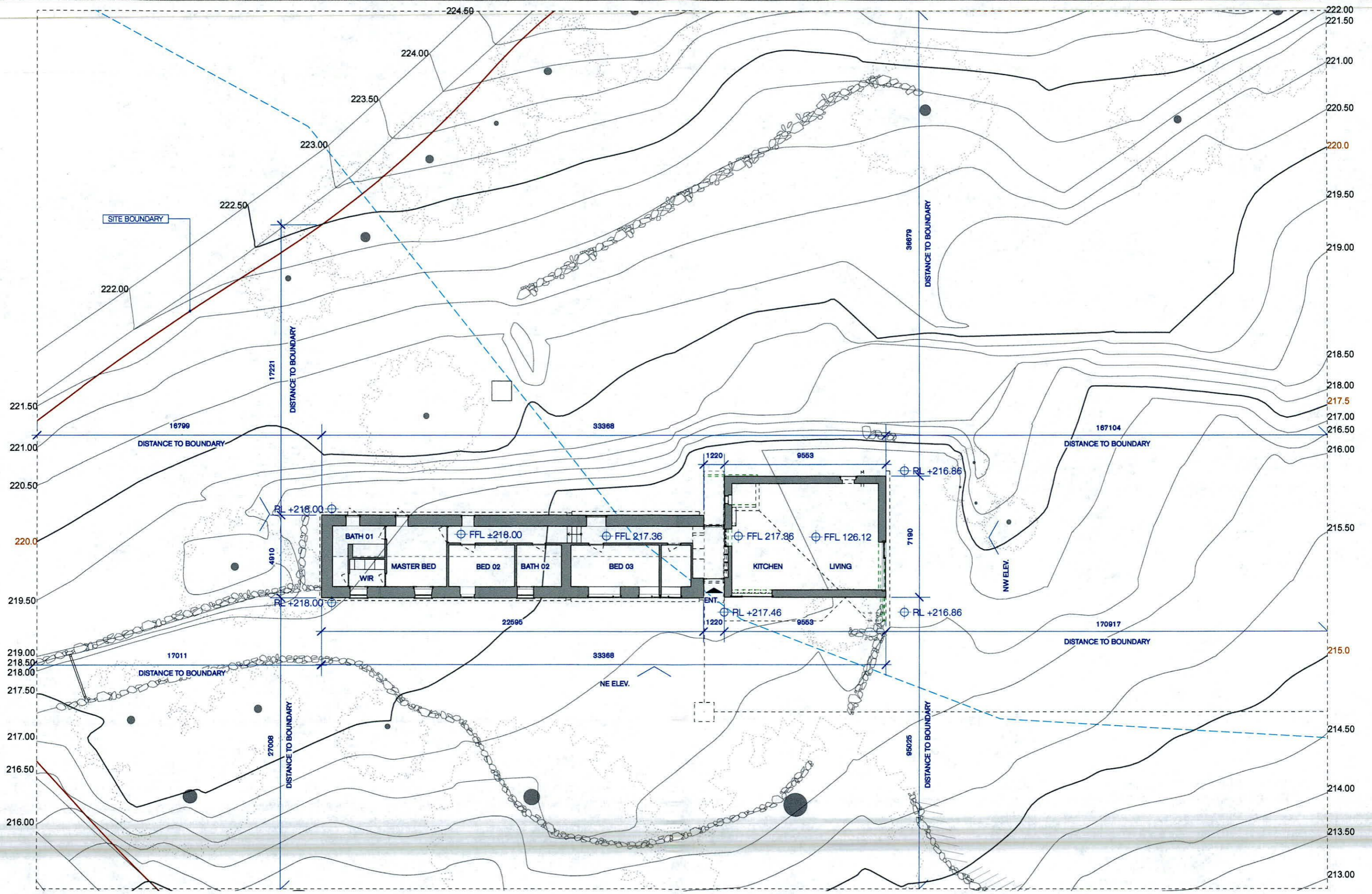
Ground Floor Plan - Existing SCALE 1: 200
