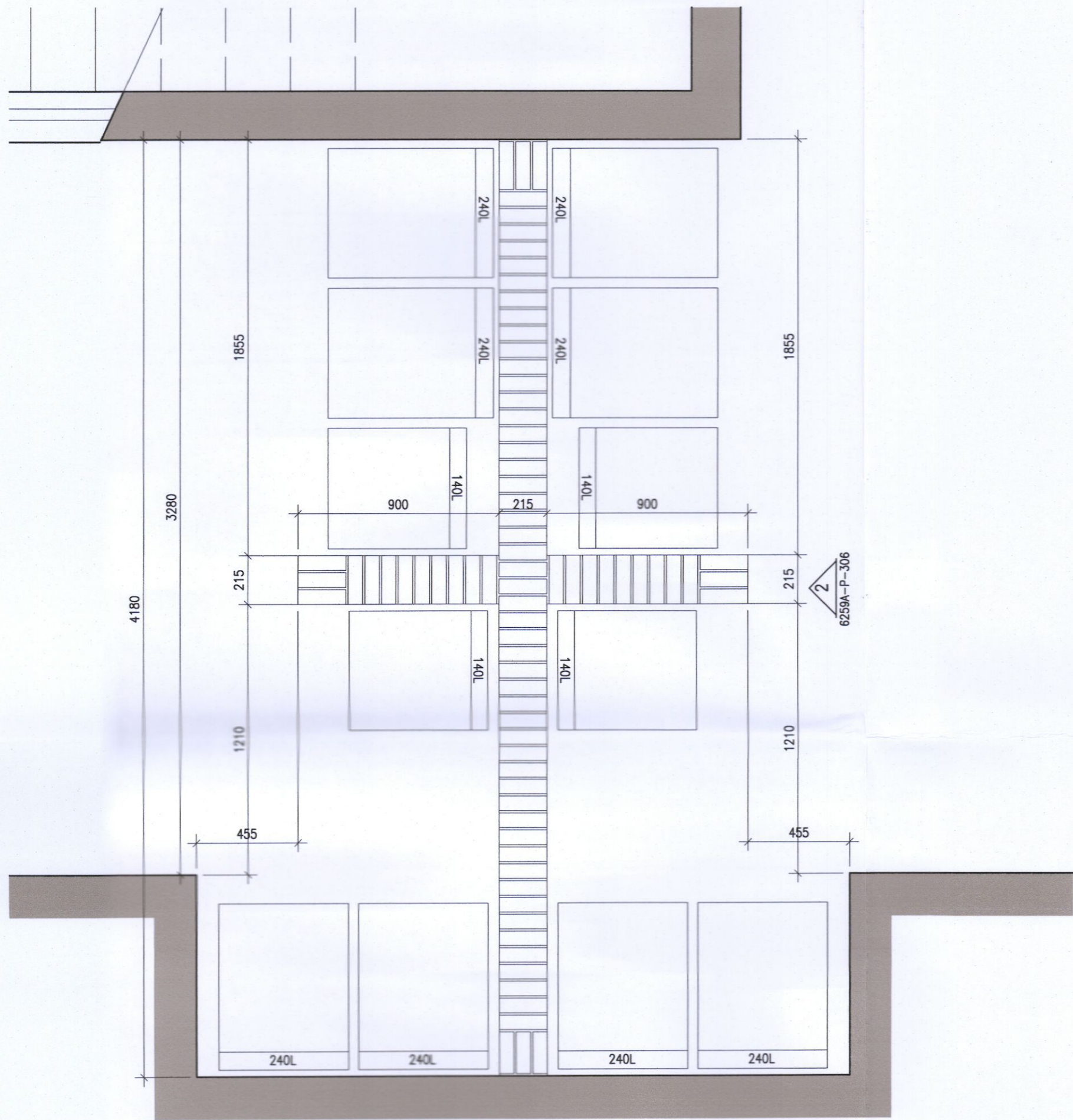
1 Bin store Type 7 Plan Scale 1:20
