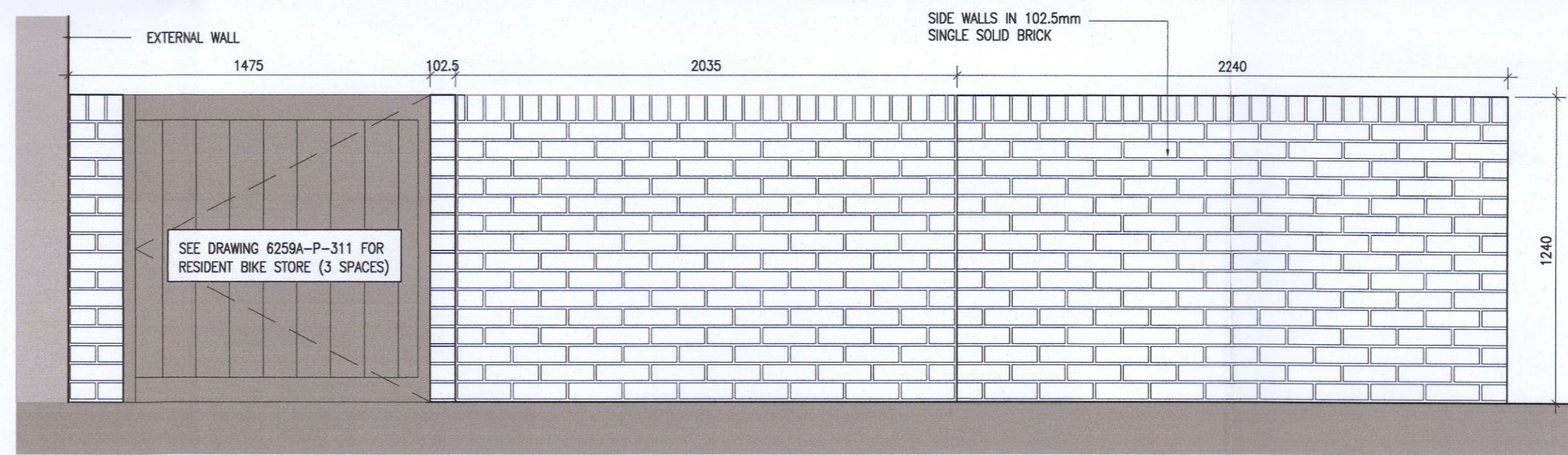
2 Bin store Type 8 Front Elevation Scale 1:20
