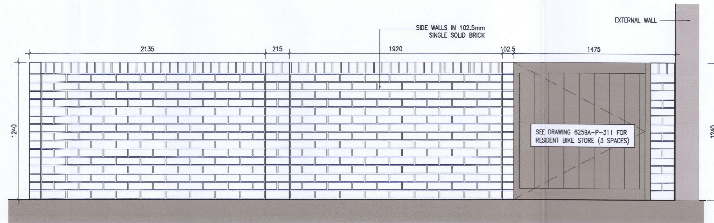
3 Bin store Type 8 Rear Elevation Scale 1:20
