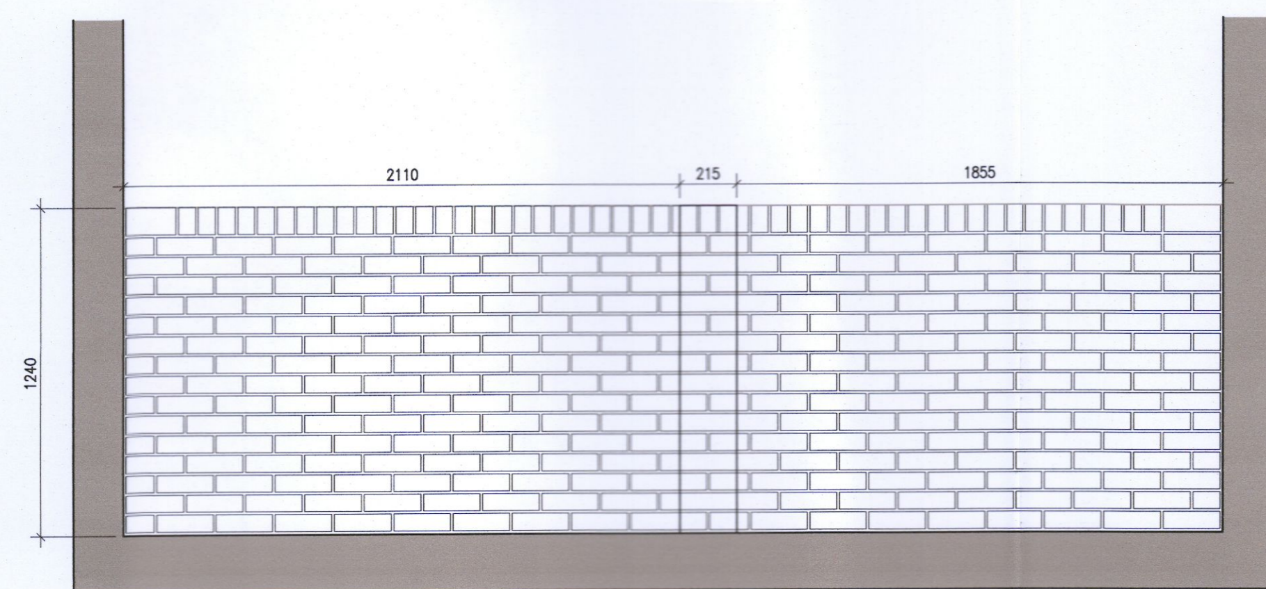
2 Bin store Type 7 Front Elevation Scale 1:20
