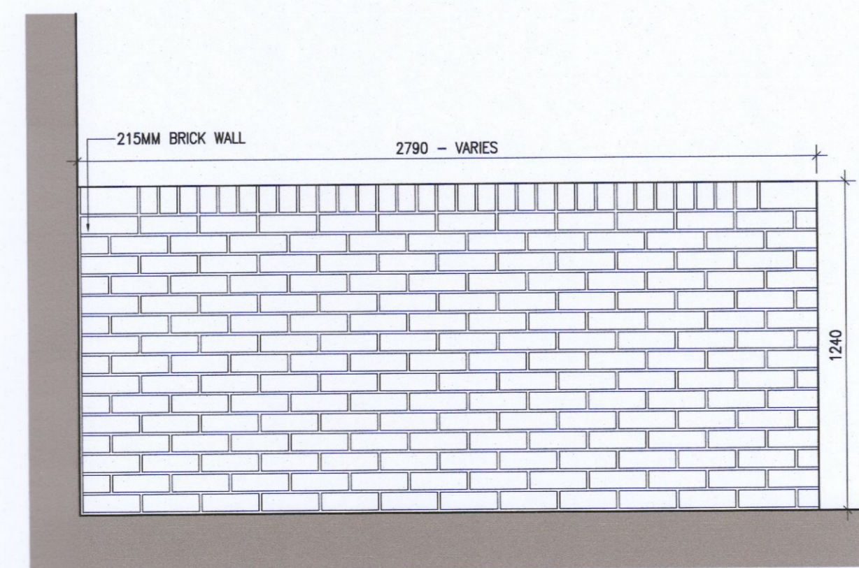
4 Bin store Type 5 Rear Elevation Scale 1:20
