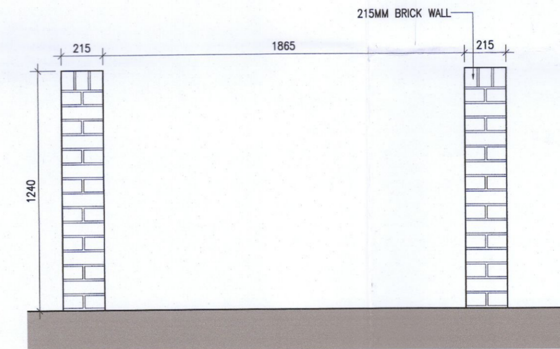
2 Bin store Type 6 Front Elevation Scale 1:20
