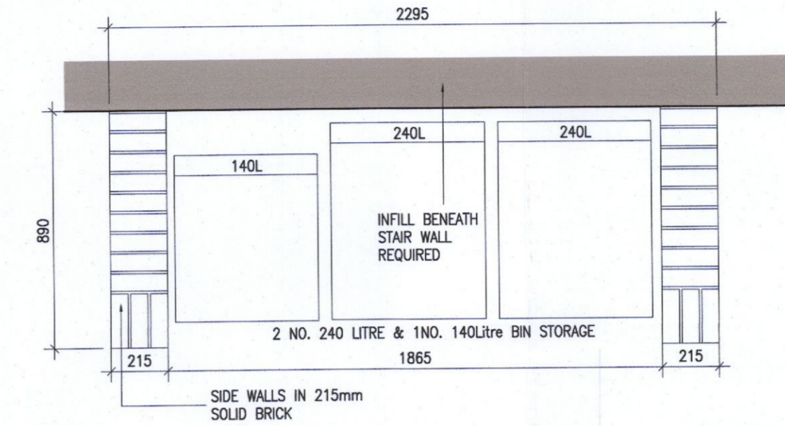
1 Bin store Type 6 Plan Scale 1:20
