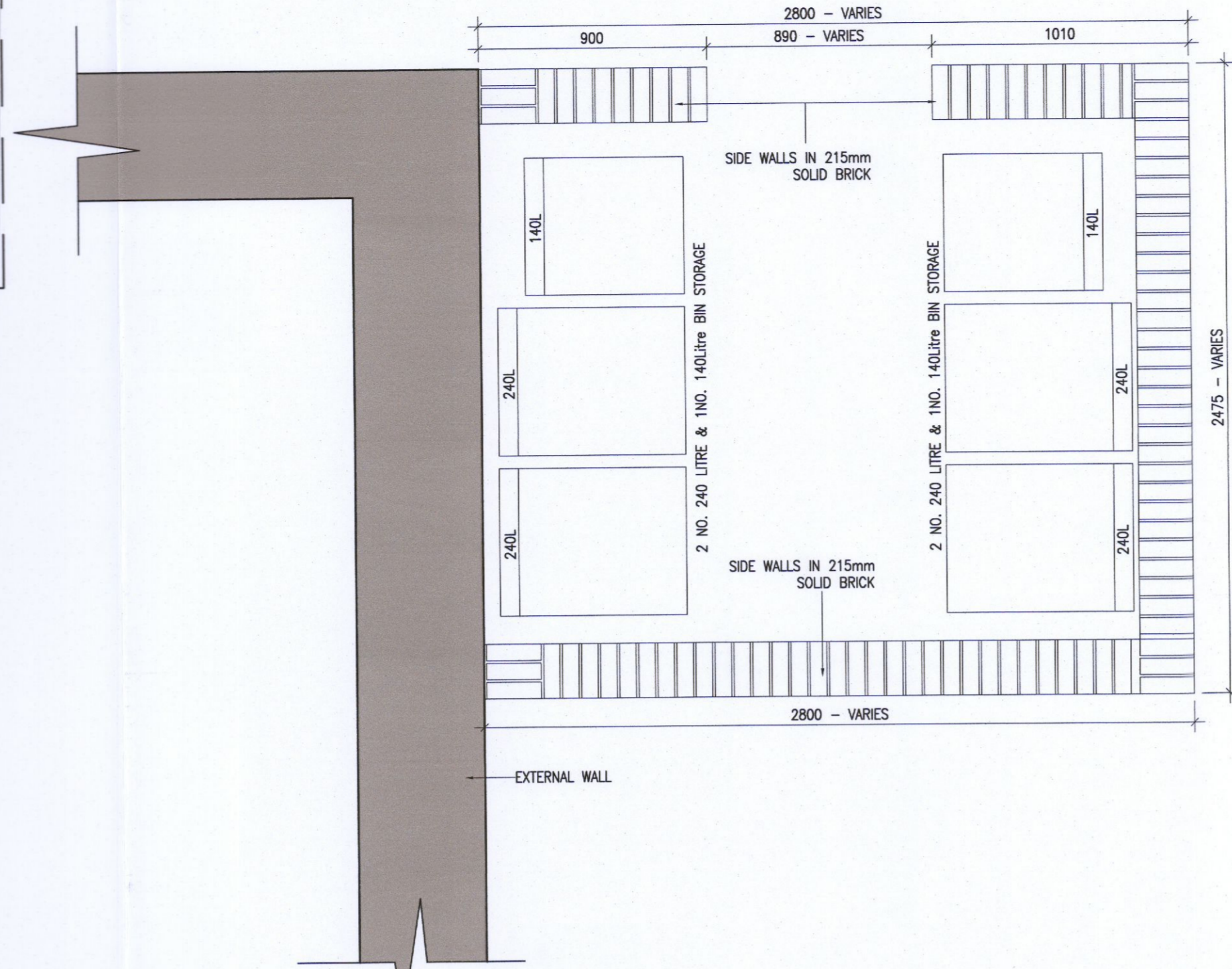
1 Bin store Type 5 Plan Scale 1:20
