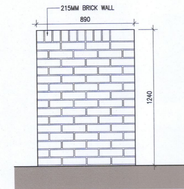
3 Bin store Type 6 Rear Elevation Scale 1:20
