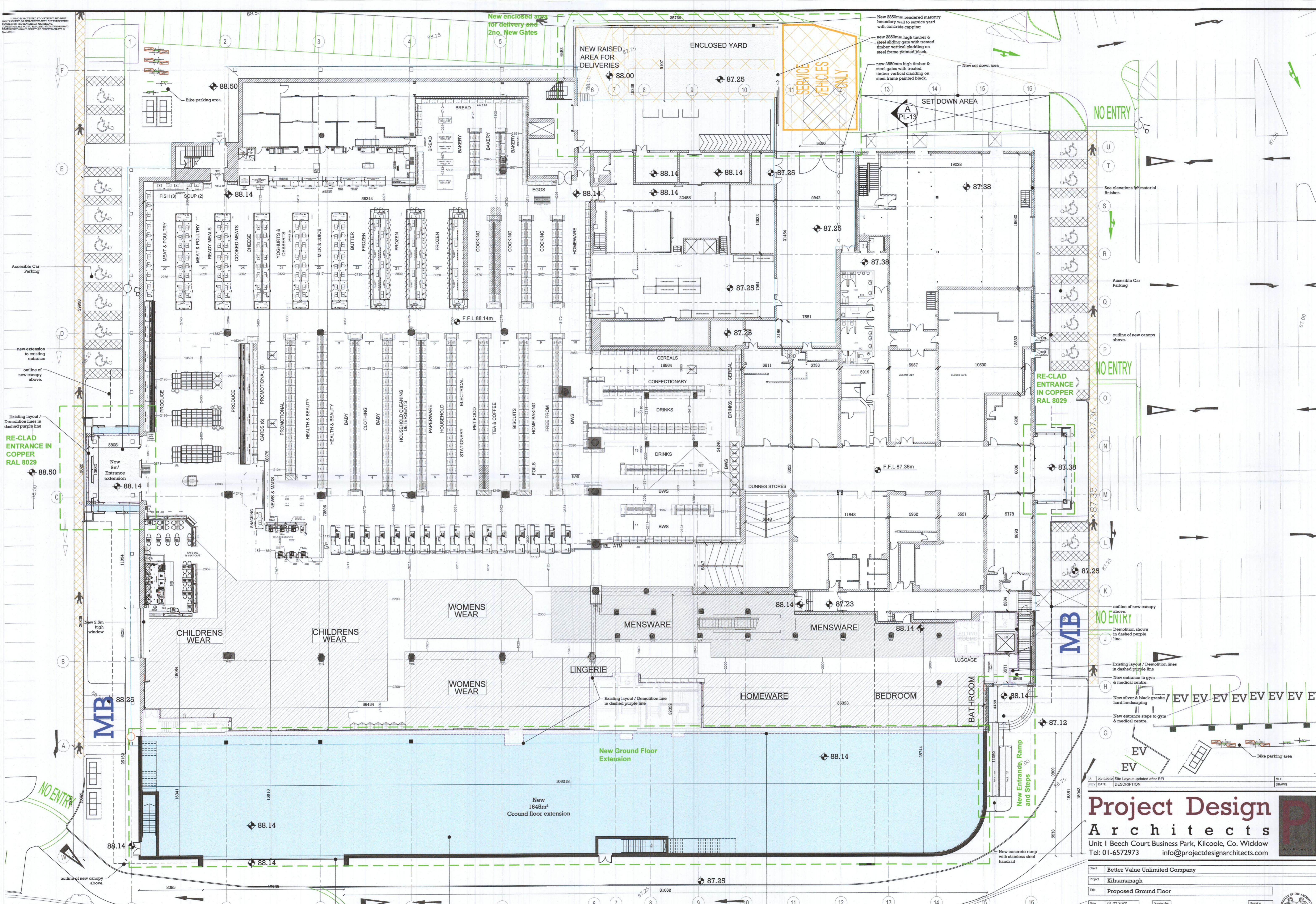
PROPOSED GROUND FLOOR PLAN SCALE: 1:200 @ A1
