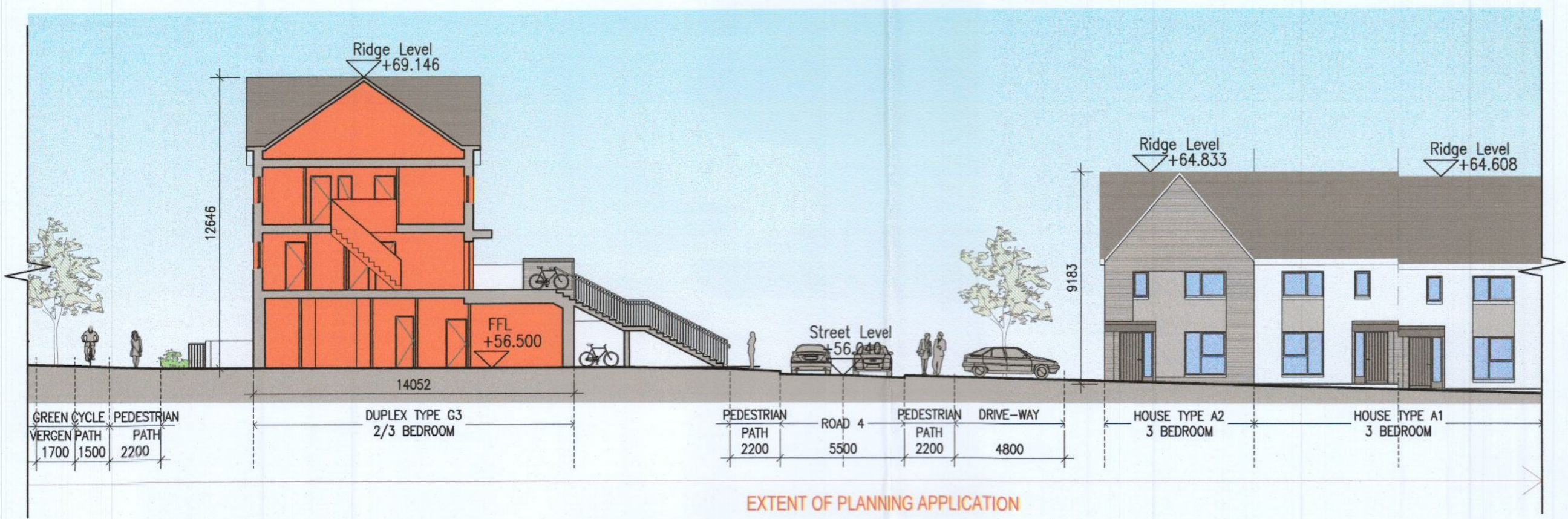
03-B P009 Site Section 03 - Part 2 1:200 @ A1
