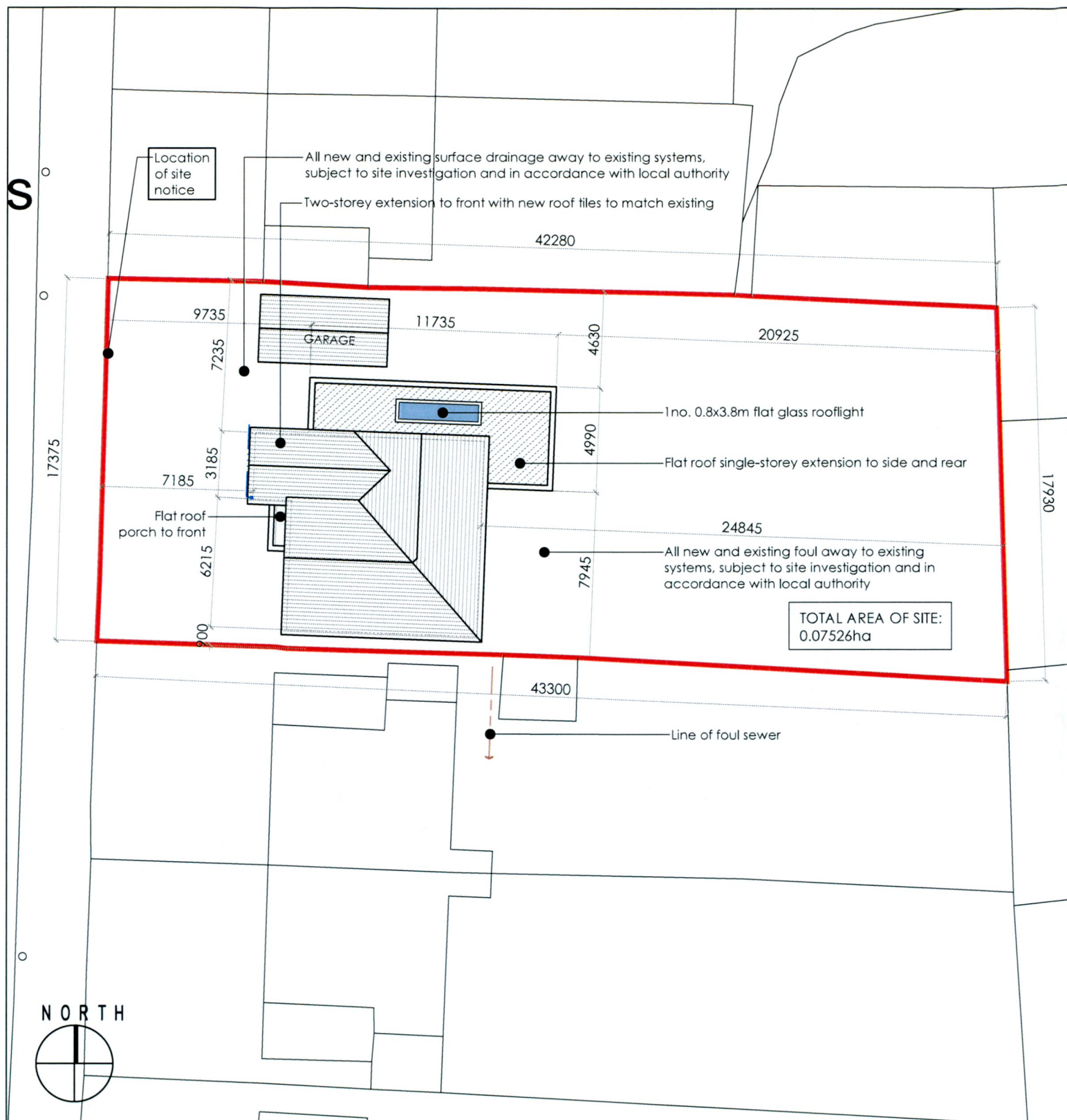
SITE LAYOUT PLAN AS PER SD19B/0332 | LICENCE NO: 25327613 | 3391-07 | 3391-08 | DN022 | X,Y: 713498,728092 scale 1:250 @ A3
