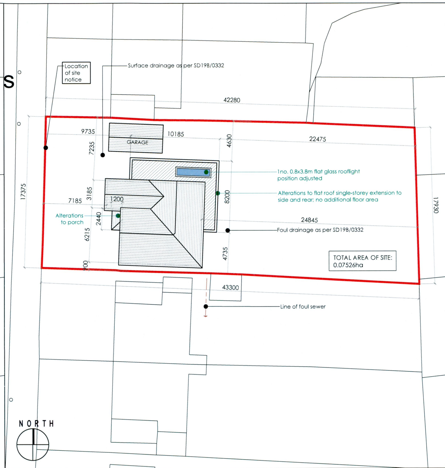
SITE LAYOUT PLAN AS BUILT | LICENCE NO: 25327613 | 3391-07 | 3391-08 | DN022 | X,Y: 713498,728092 scale 1:250 @ A3
