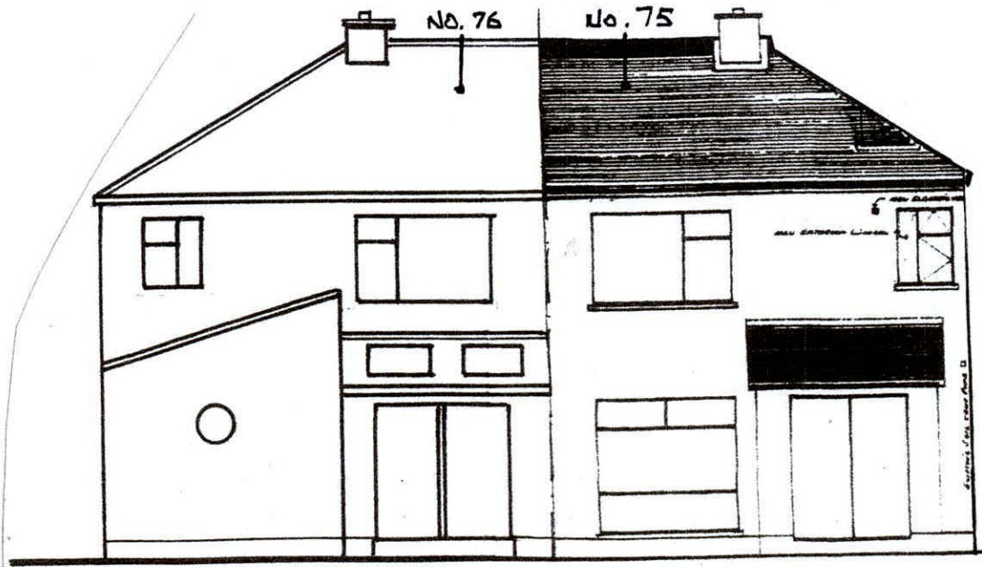
REAR CONTIGUOUS ELEVATION
