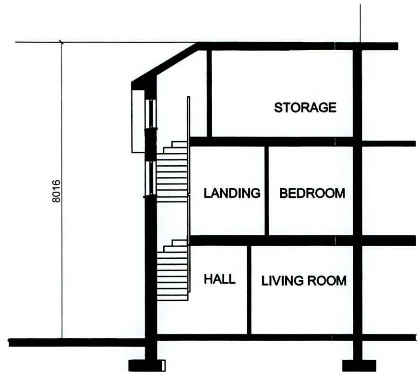
SECTION B-B
